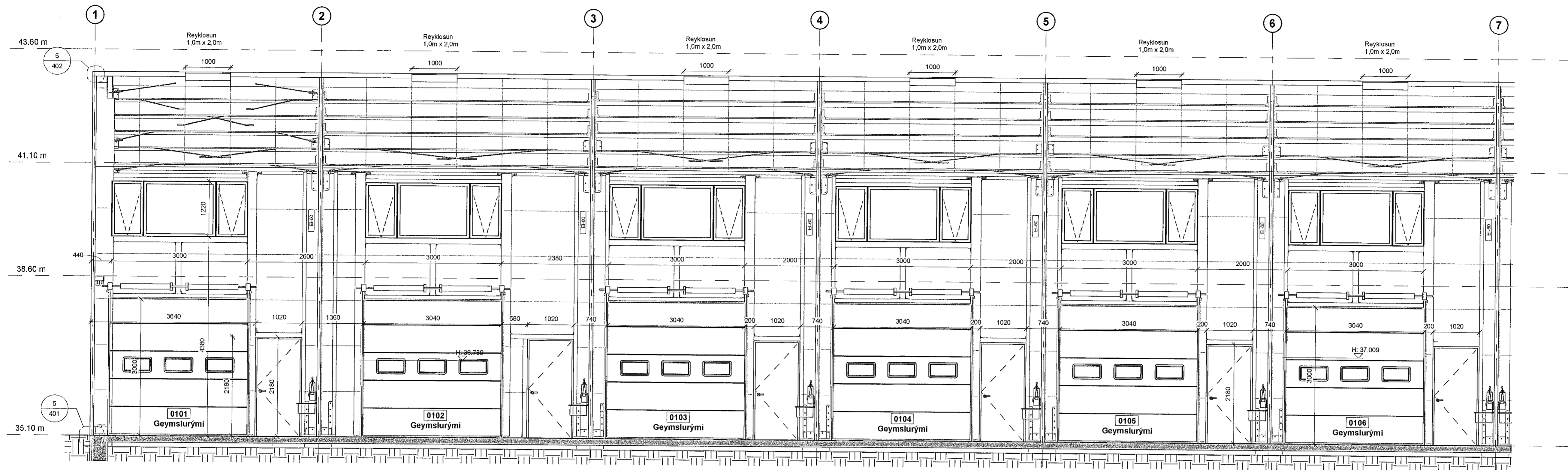
- SNID C - Hluti 1-7 1 : 50
