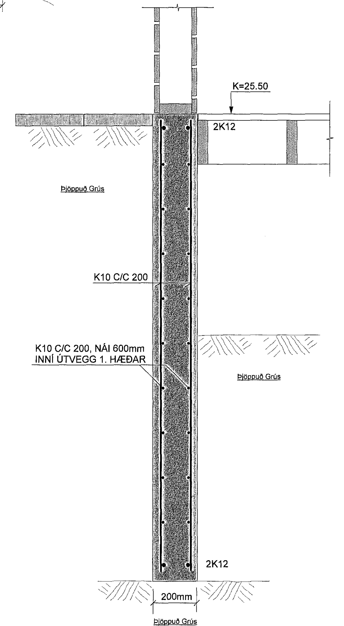
SNID H-H MKV. 1:10
