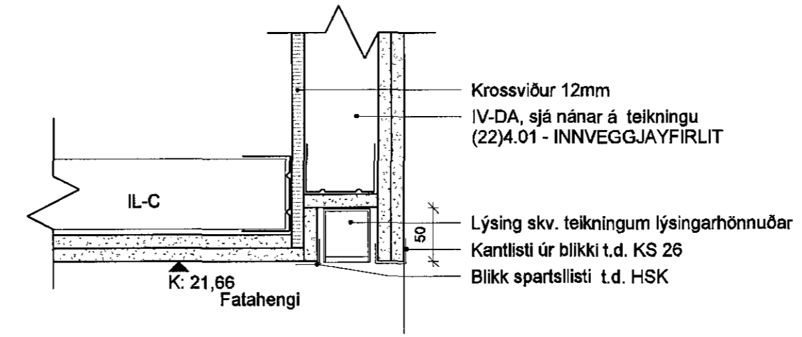
3 (45) LÓ - Loft yfir fatahengi 1:5
