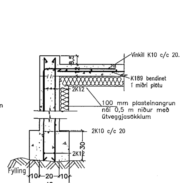
D SNID D-D. 1:20.
