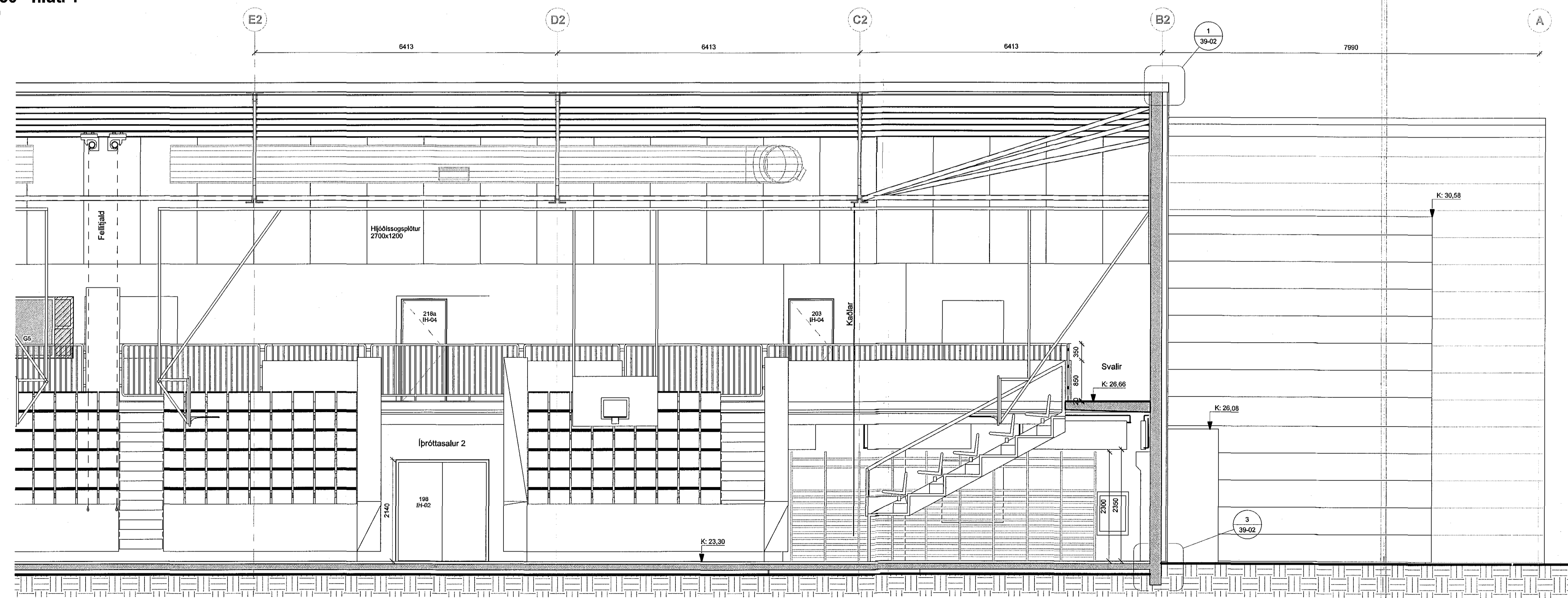
F-F 50 - hluti 2 1 : 50
