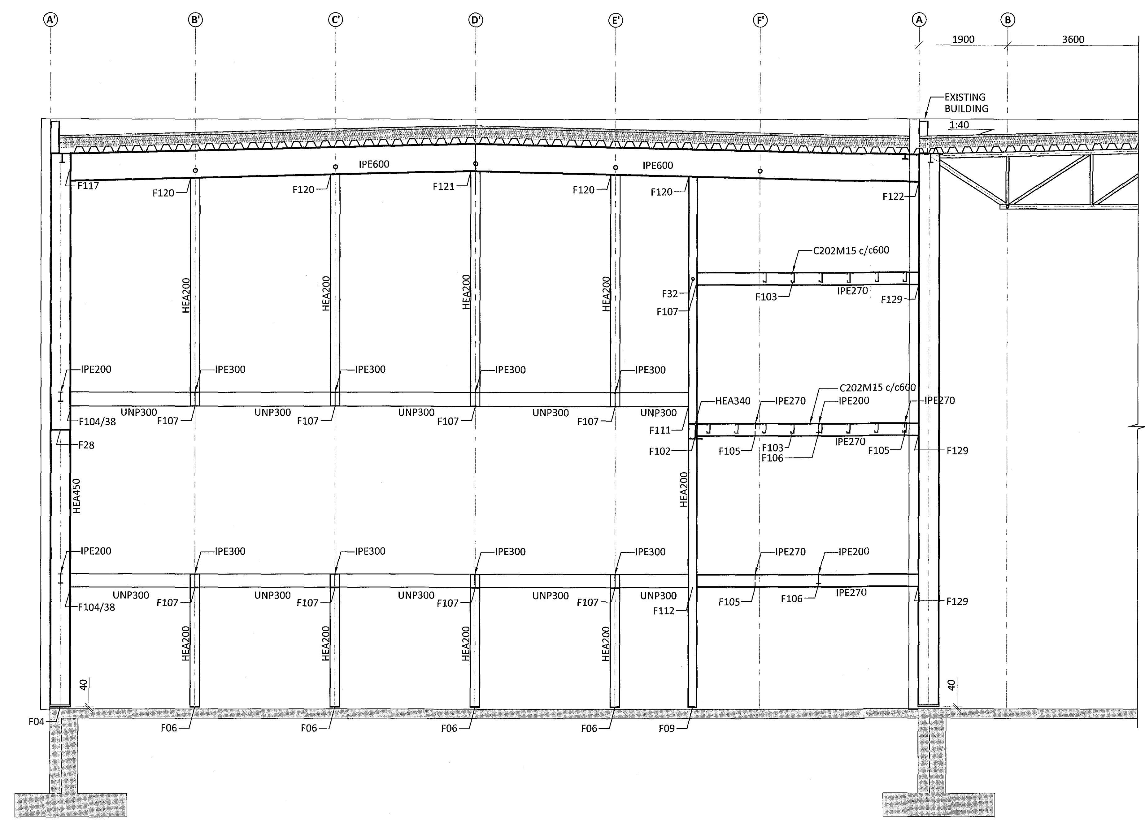
SECTION VIEW GRIDLINE 11 SC1:50
