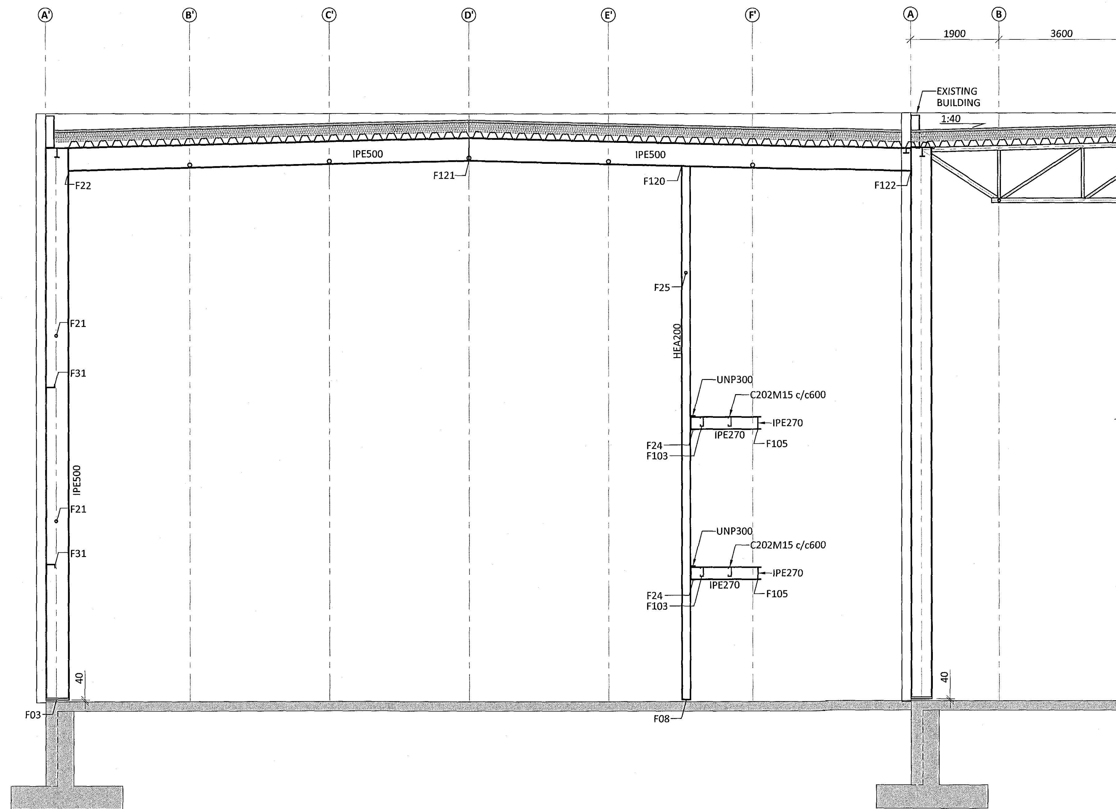
SECTION VIEW GRIDLINE 5 SC1:50
