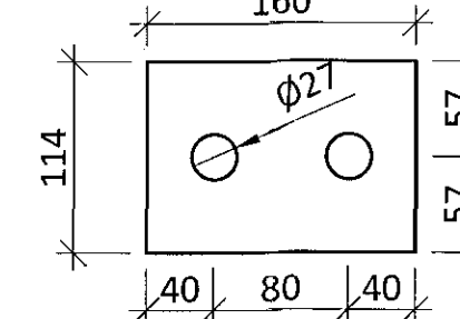
STEEL PLATE S054 - t=20mm - M1:5 S355
