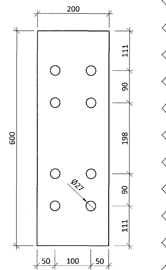
STEEL PLATE S055 - t=15mm - M1:5 S355
