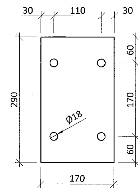
STEEL PLATE S056 - t=10mm - M1:5 S355
