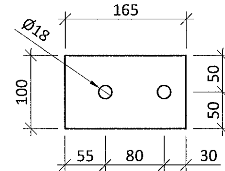
STEEL PLATE S037 - t=10mm - M1:5 S355
