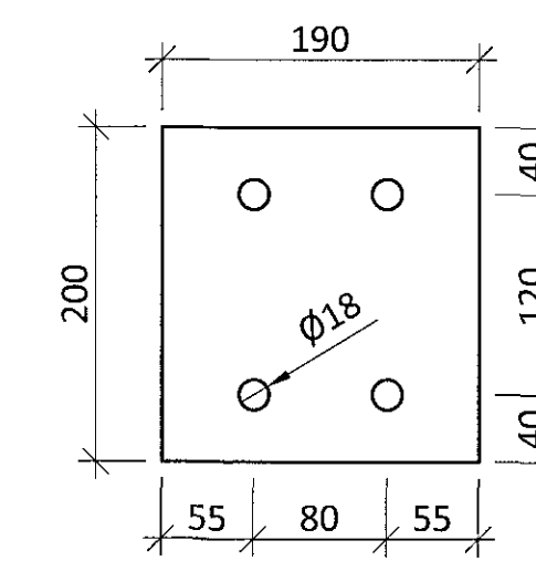
STEEL PLATE S046 - t=15mm - M1:5 S355
