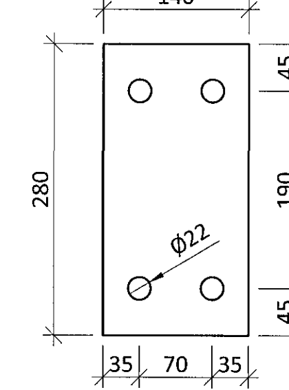
STEEL PLATE S052 - t=20mm - M1:5 S355
