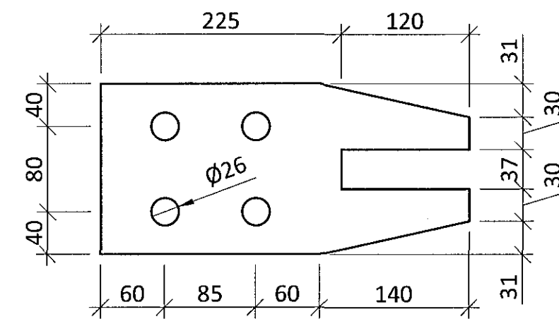
STEEL PLATE S047 - t=20mm - M1:5 S355
