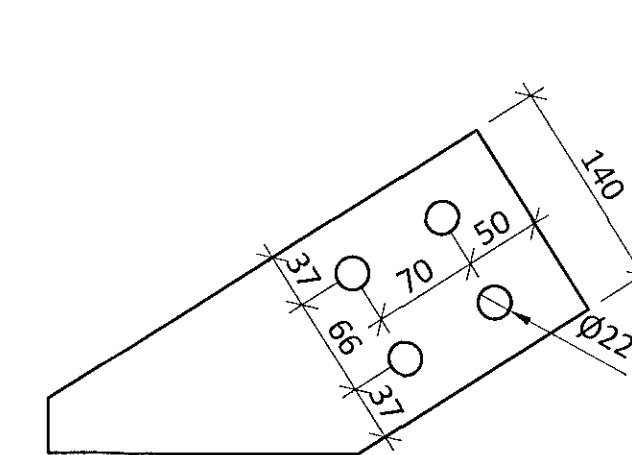
STEEL PLATE S053 - t=10mm - M1:5 S355
