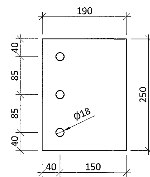
STEEL PLATE S057 - t=15mm - M1:5 S355
