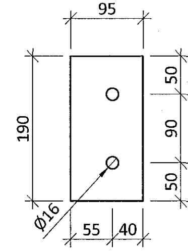
STEEL PLATE S035 - t=10mm - M1:5 S355
