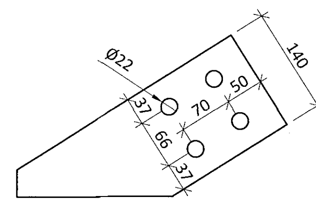
STEEL PLATE S051 - t=10mm - M1:5 S355
