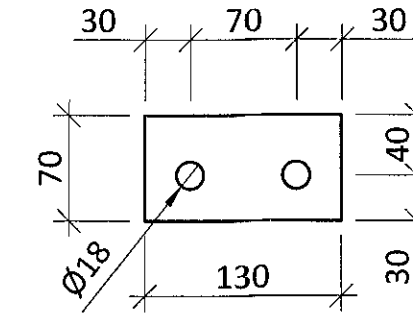
STEEL PLATE S038 - t=10mm - M1:5 S355
