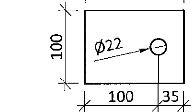
STEEL PLATE S049 - t=10mm - M1:5 S355
