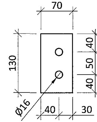
STEEL PLATE S036 - t=10mm - M1:5 S355
