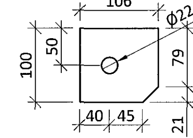
STEEL PLATE S048 - t=10mm - M1:5 S355
