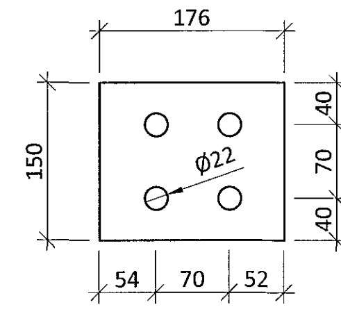
STEEL PLATE S048 - t=10mm - M1:5 S355
