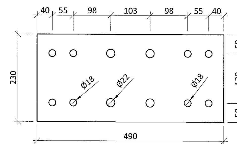
STEEL PLATE S059 - t=10mm - M1:5 S355
