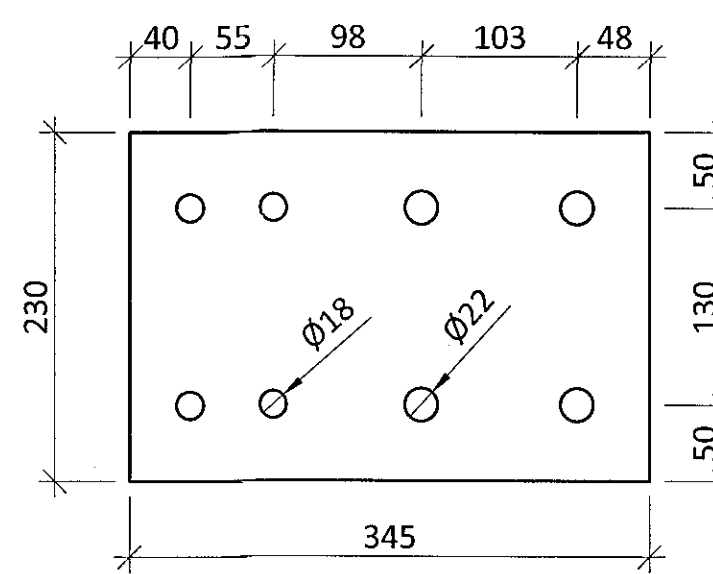
STEEL PLATE S058 - t=10mm - M1:5 S355
