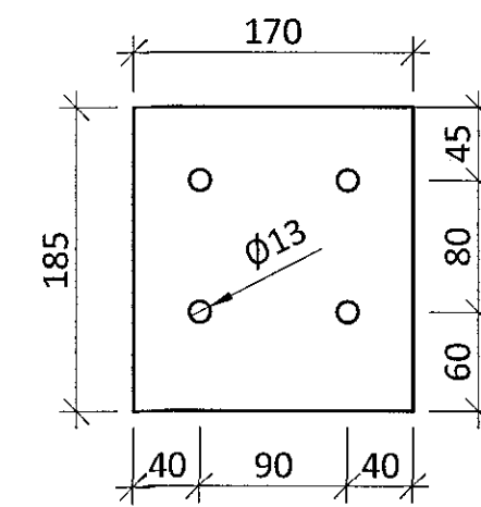
STEEL PLATE S044 - t=10mm - M1:5 S355
