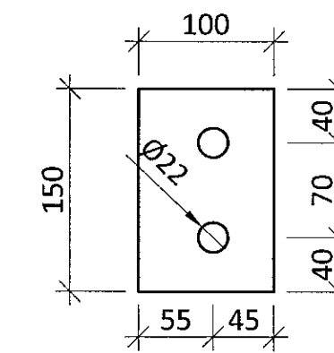
STEEL PLATE S045 - t=10mm - M1:5 S355
