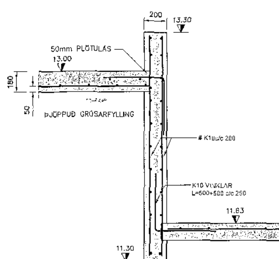
SNIB R 1:20
