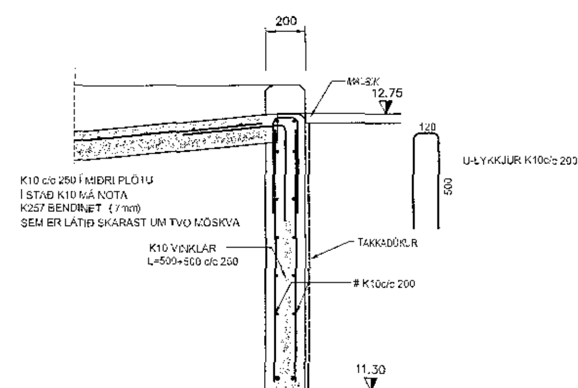
SNIB Q 1:20
