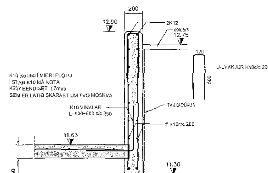
SNIB T 1:20
