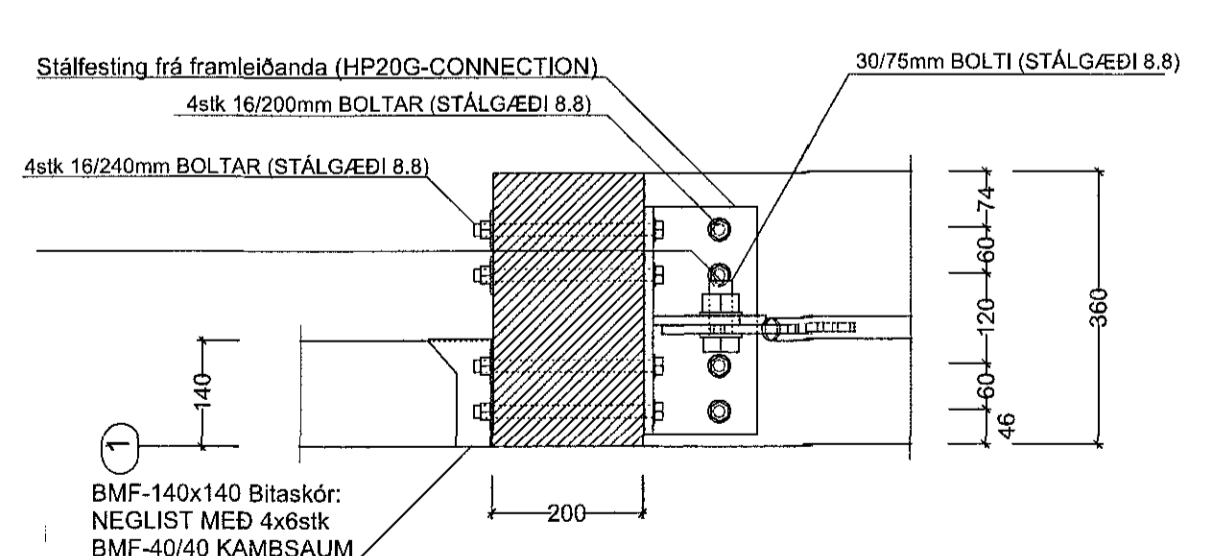
SNID V3/V4 - 7A MKV. 1:10
