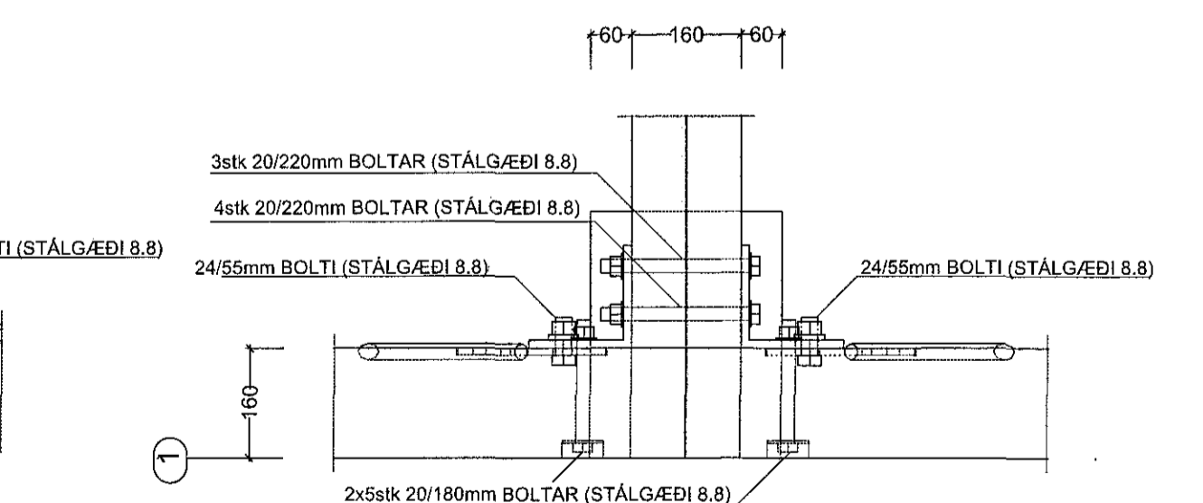
SNID V3/V4 - 6A MKV. 1:10
