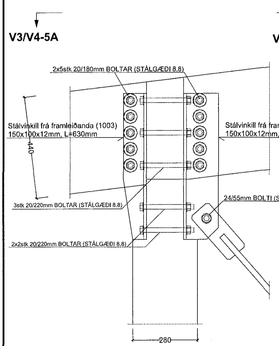
SNID V3/V4 - 5A MKV. 1:10
