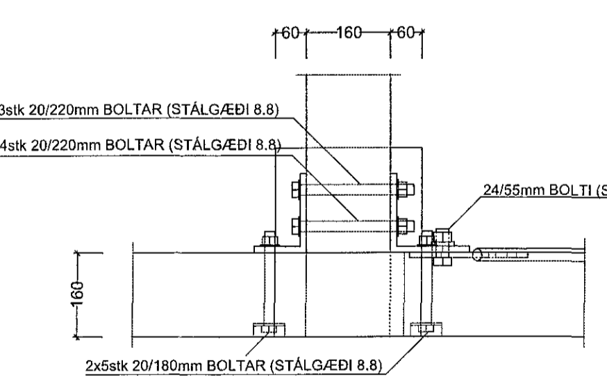
SNID V3/V4 - 5A MKV. 1:10
