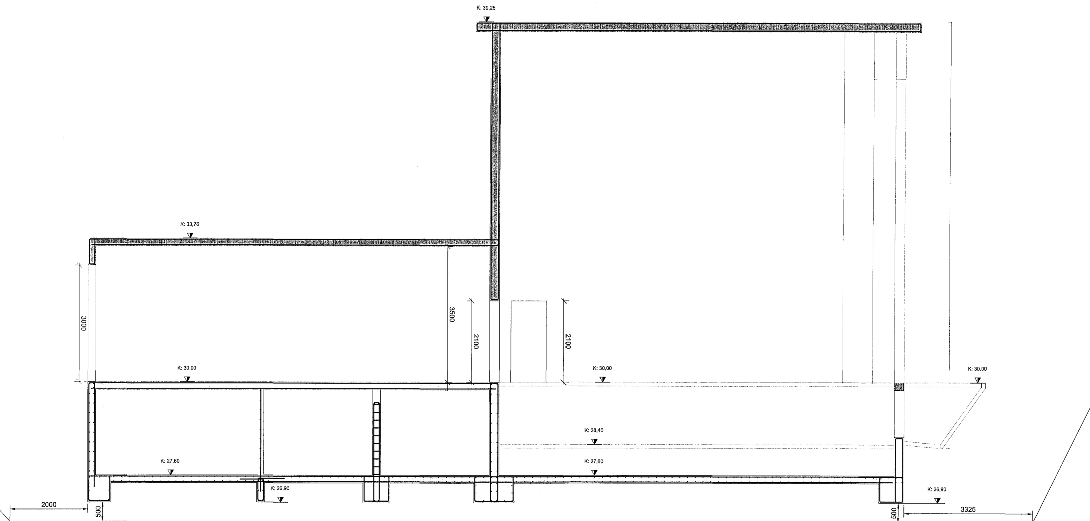
1 SNID 3.111 | 3.211 | 1:50
