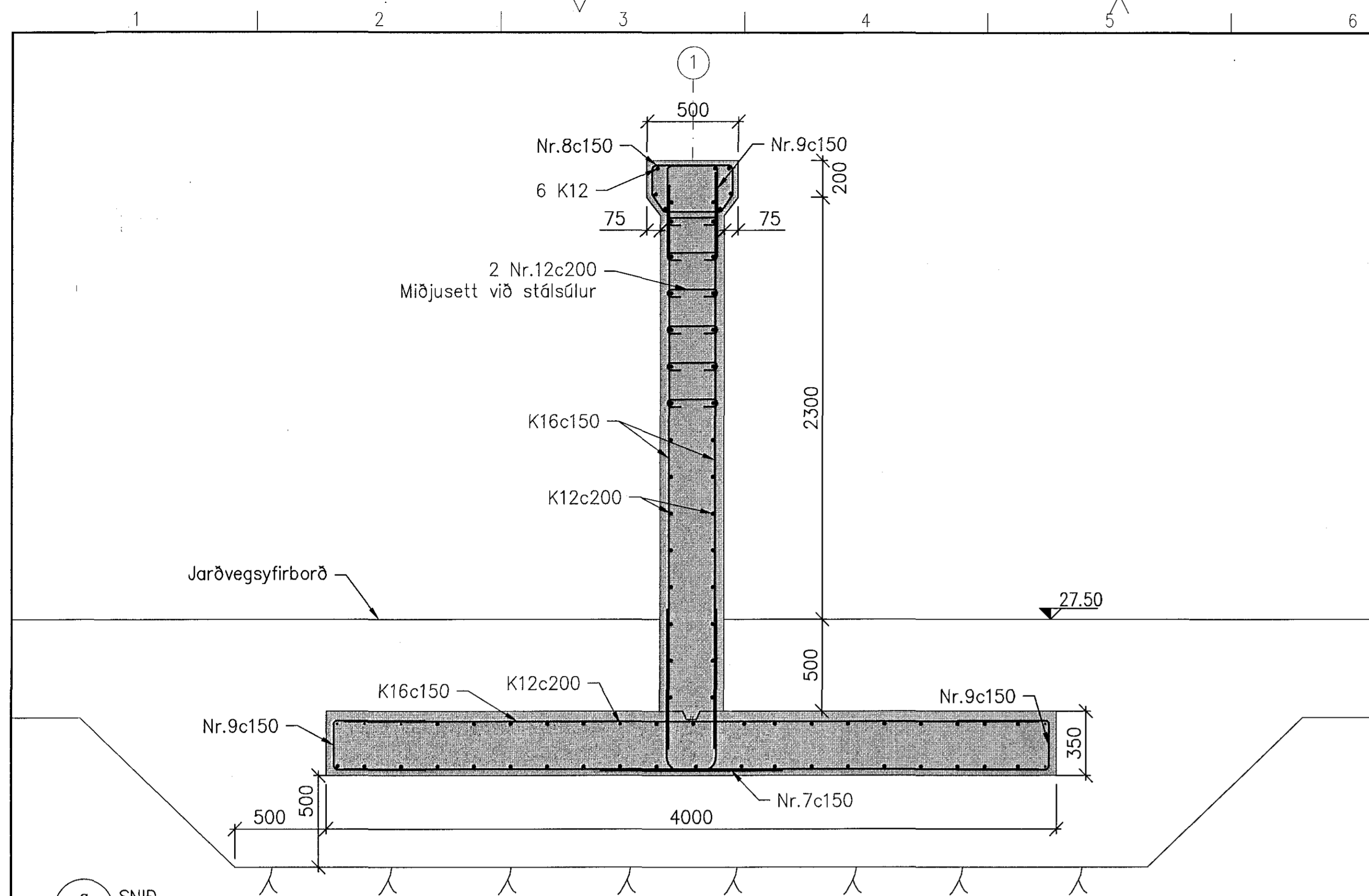
a SNID 102 1:20
