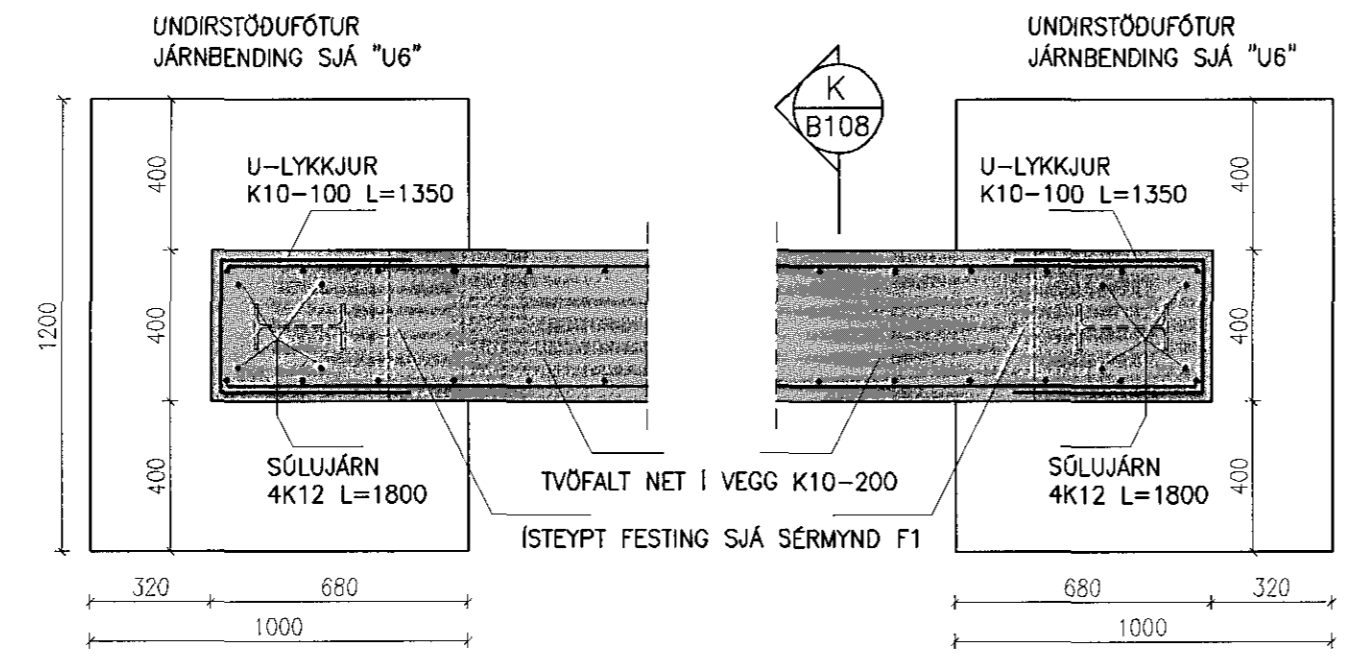
SNID 23-23 1:20
