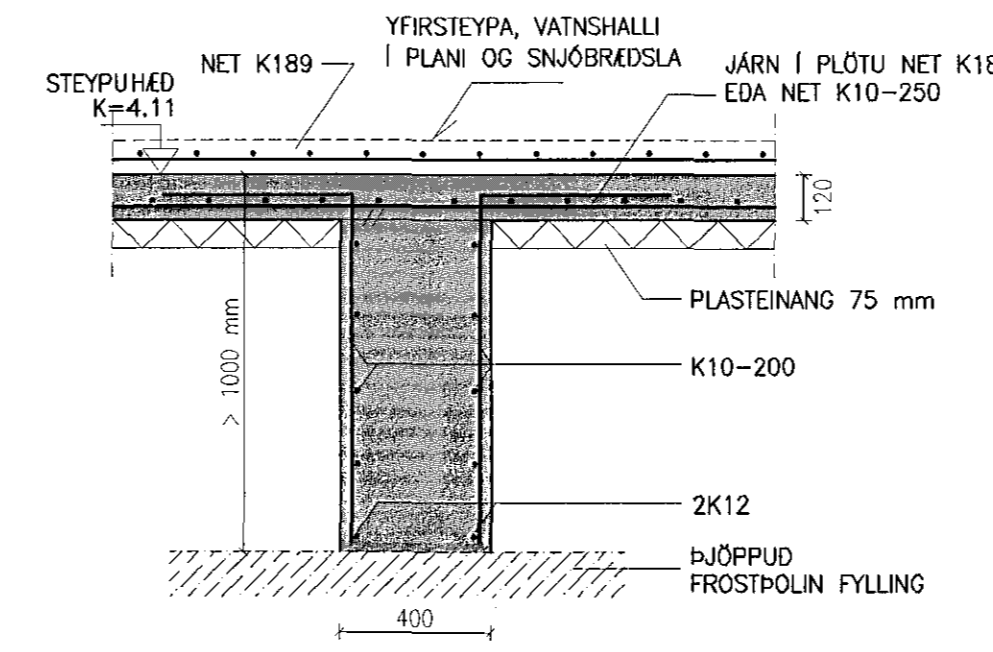
SNID K-K 1:20
