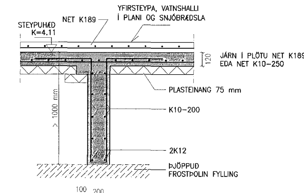
SNID 24-24 1:20
