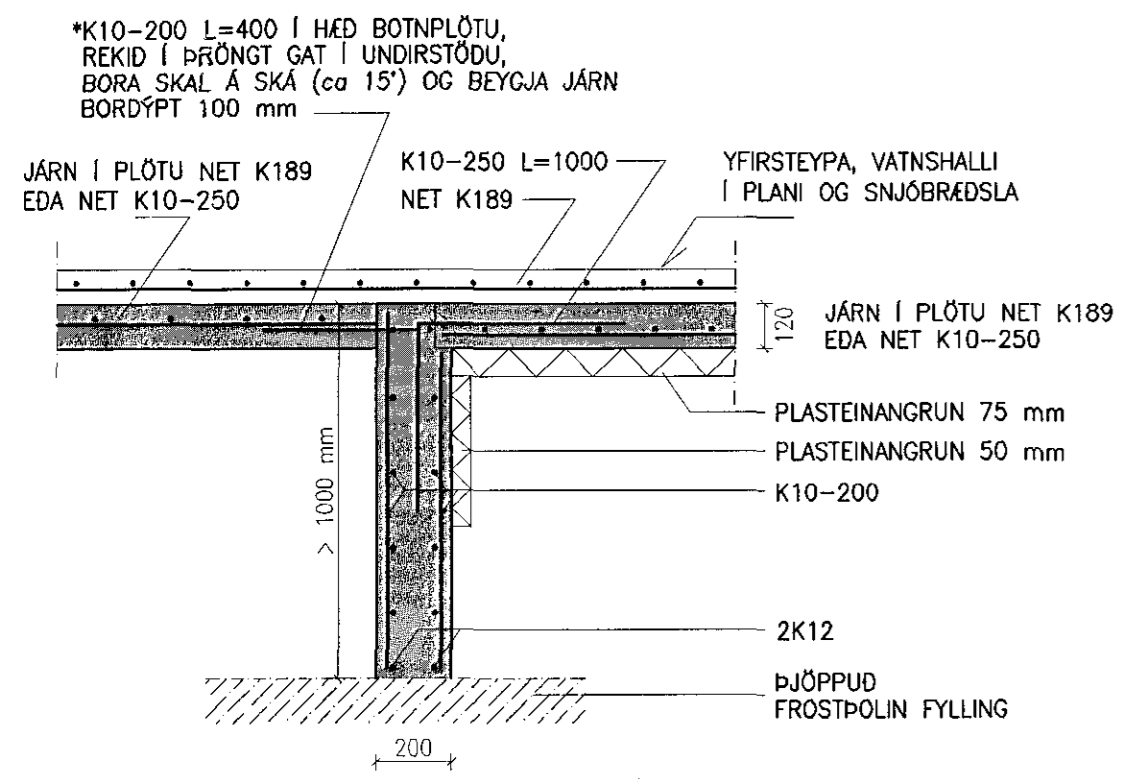
SNID 22-22 1:20
