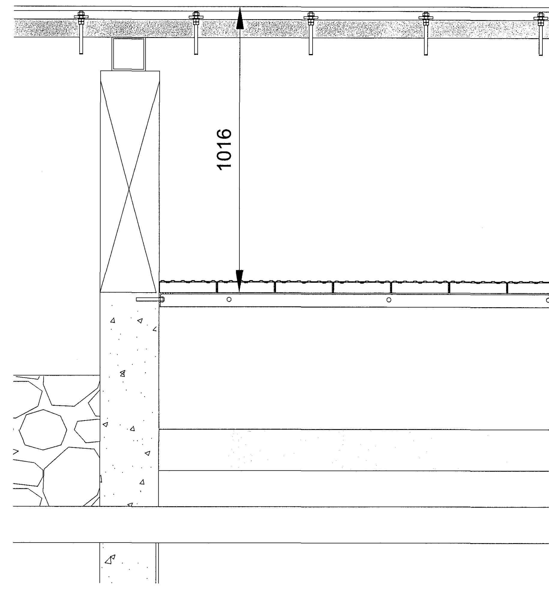
1 SNID 1 C.2.121 2.121 1:8
