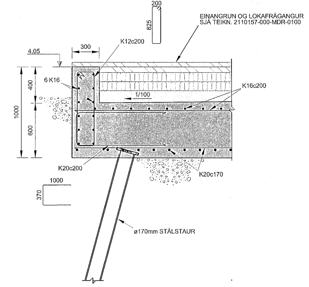
A SNID 1:20
