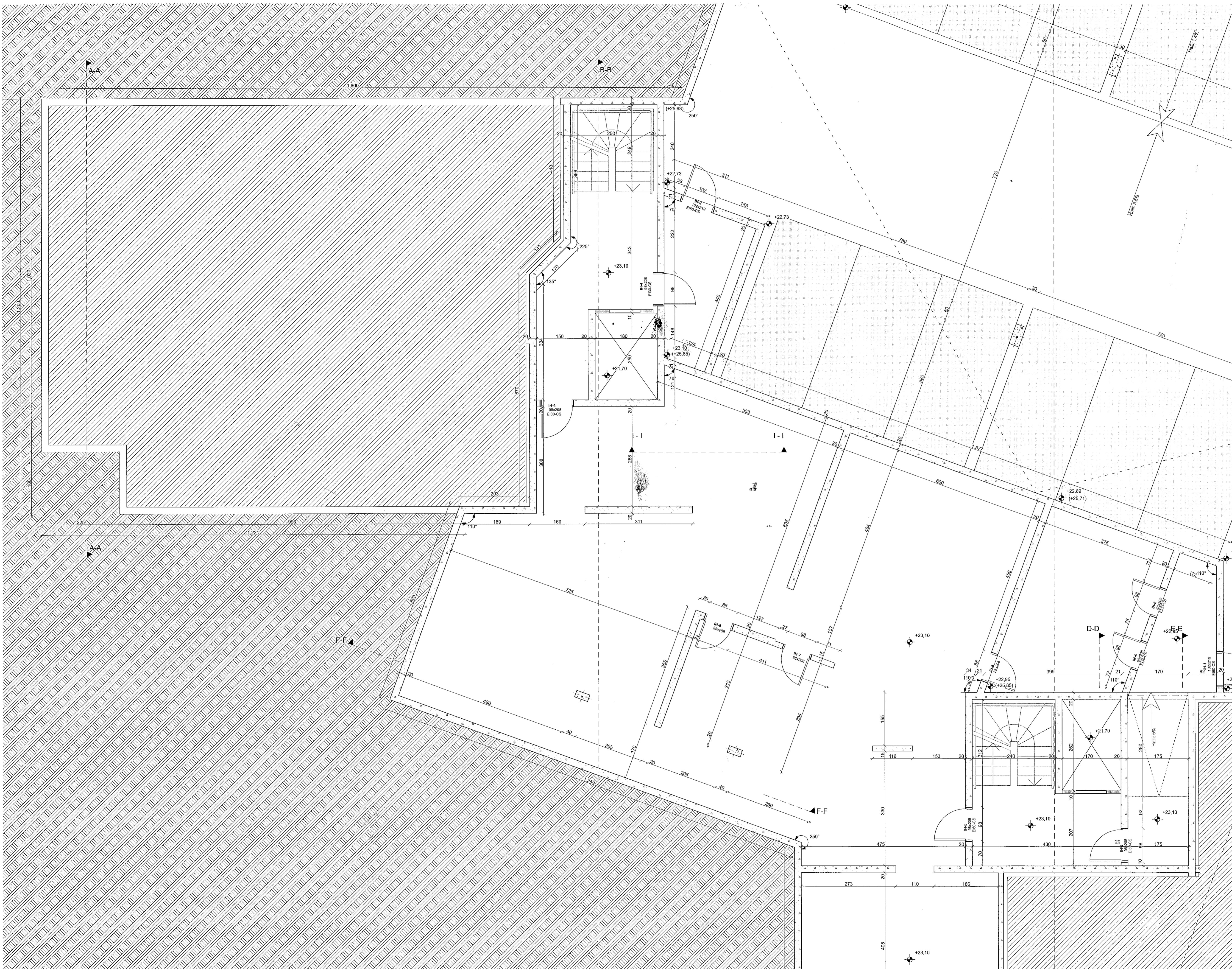
0. kjallari
