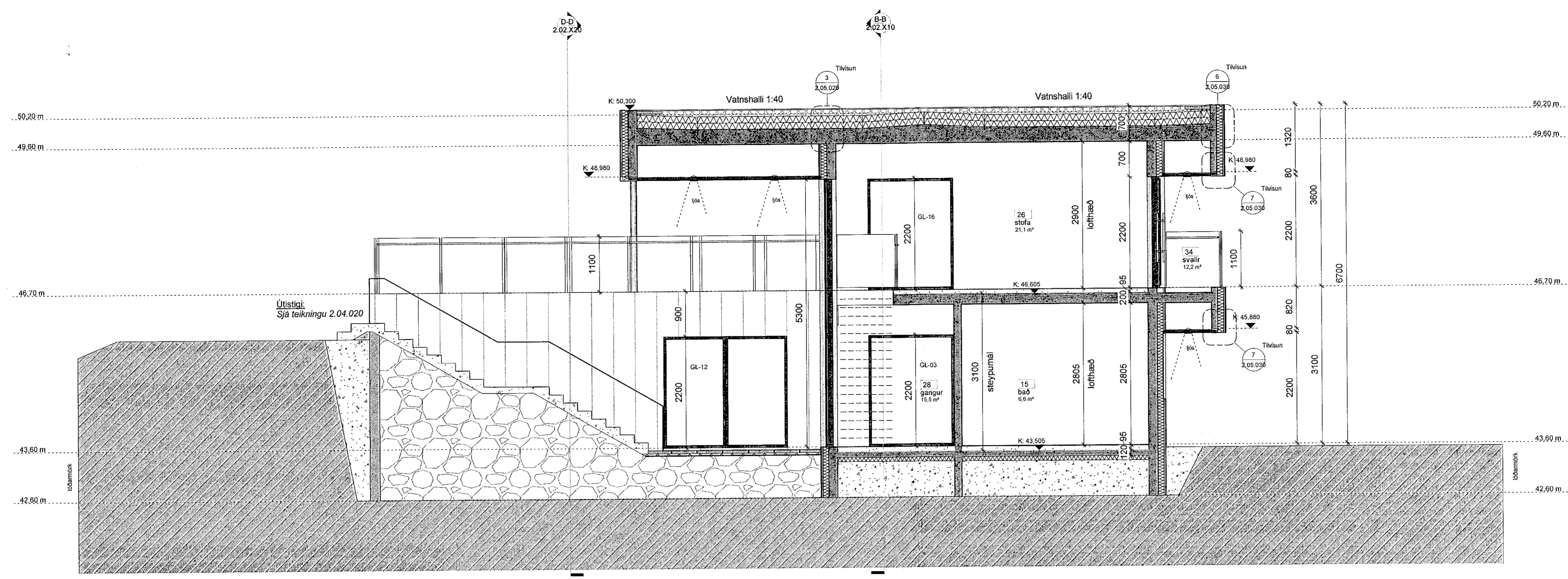
6.0-SNEIDING F-F 1:50
