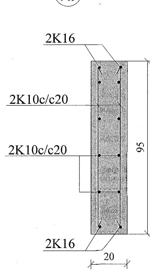
C5 SNID. 1:10
