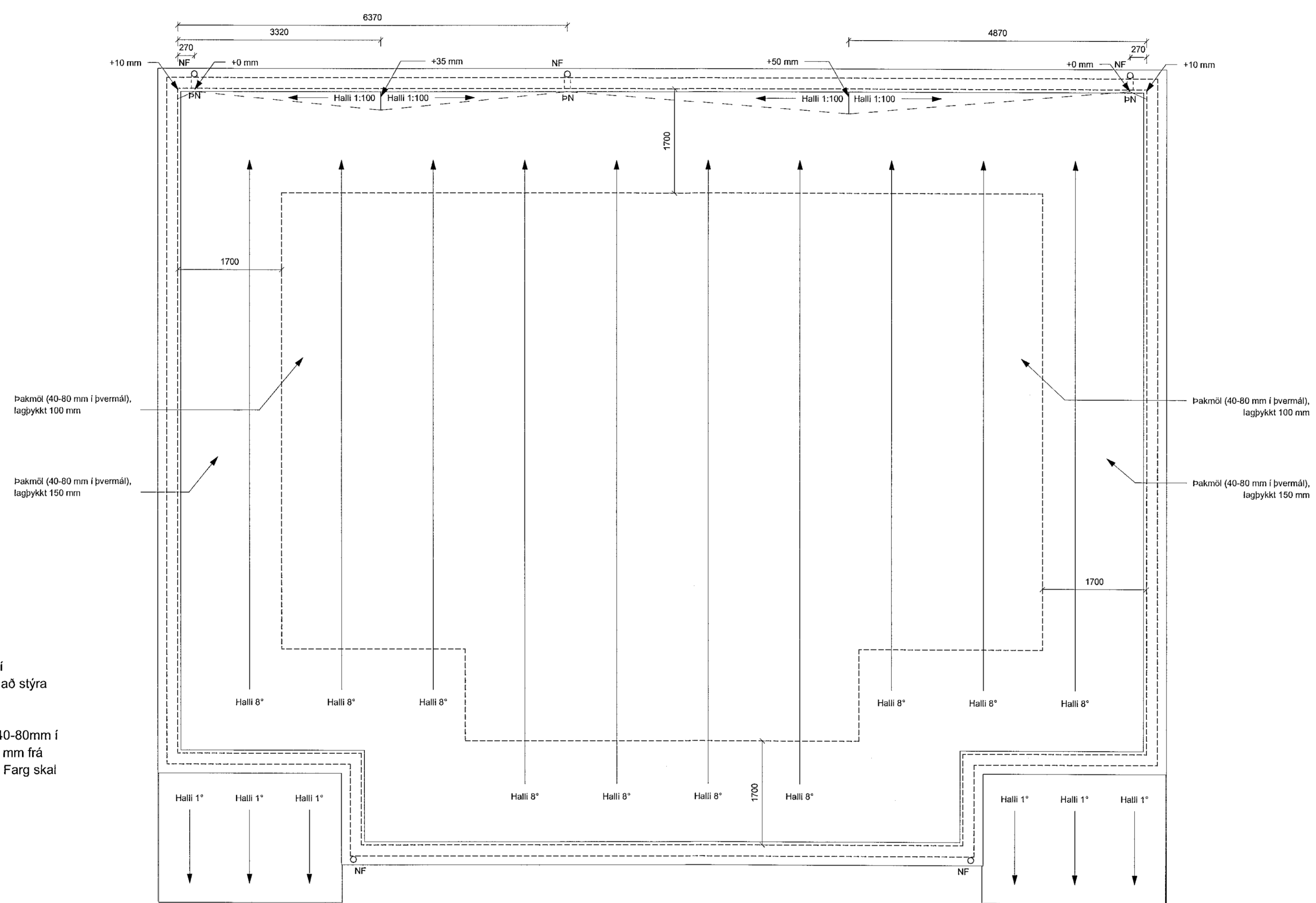
ÞAKHALLAPLAN mkv: 1 : 50
