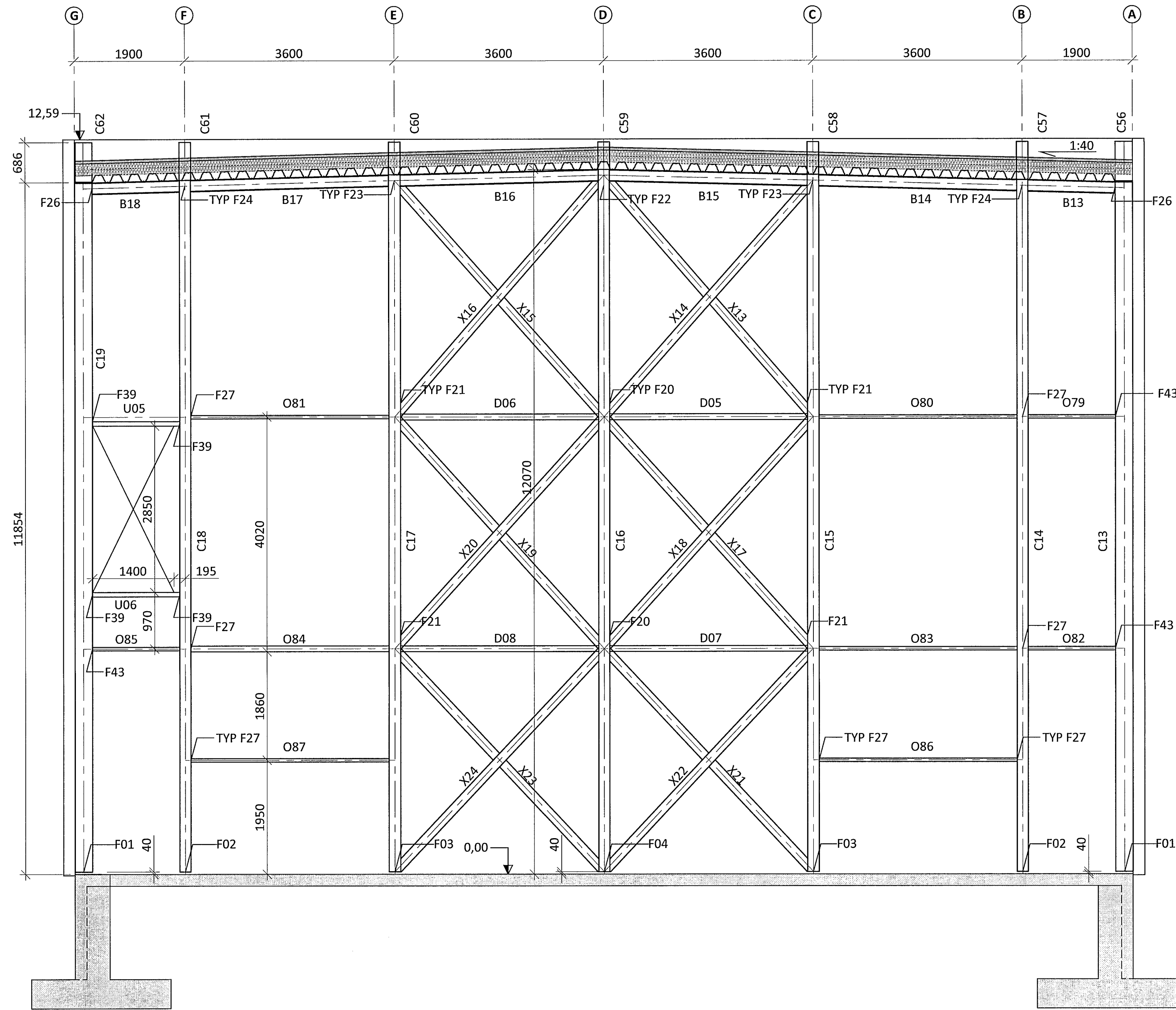
ELEVATION VIEW GRIDLINE 13 SC1:50
