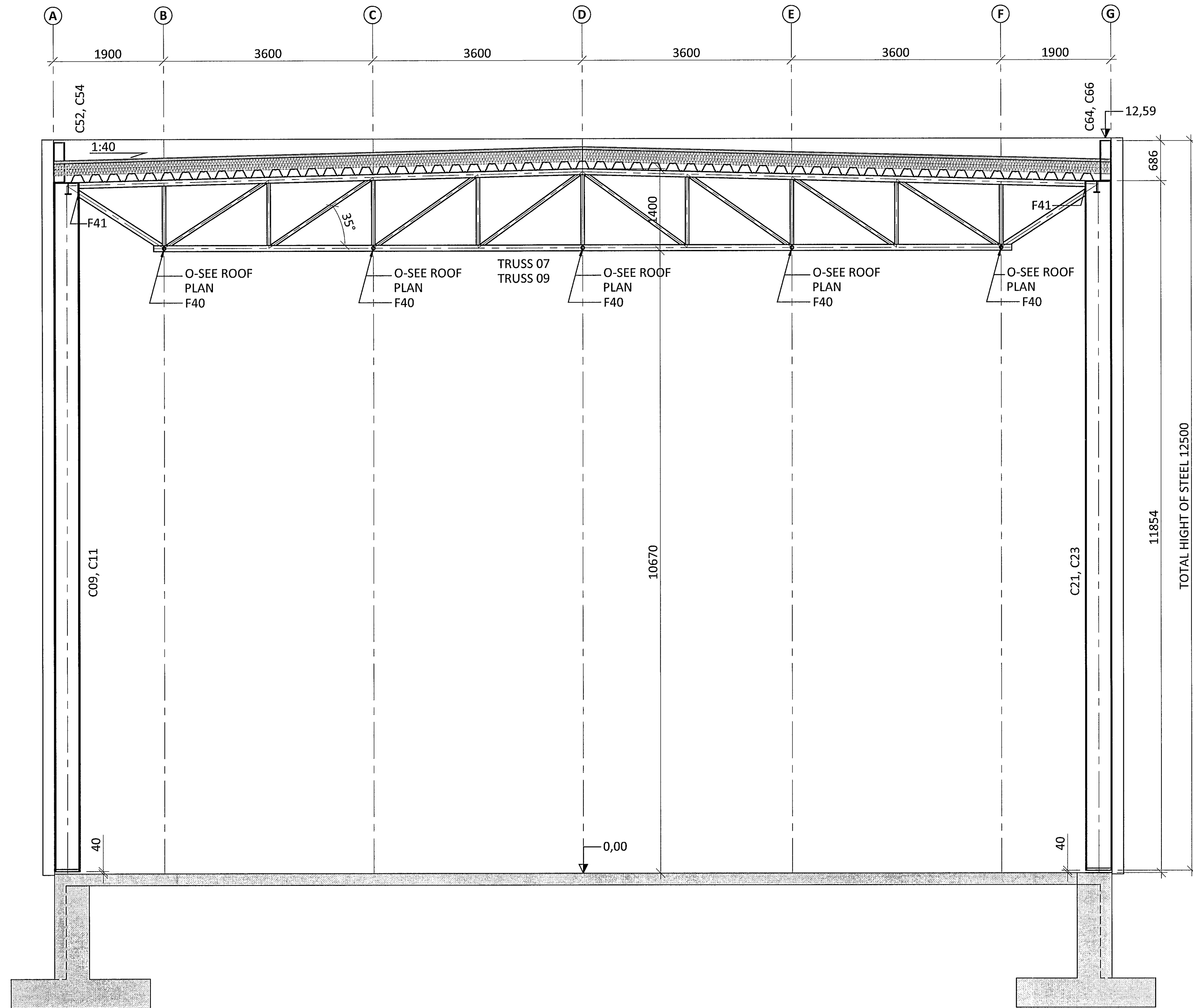
SECTION VIEW GRIDLINES 9 AND 11 SC1:50
