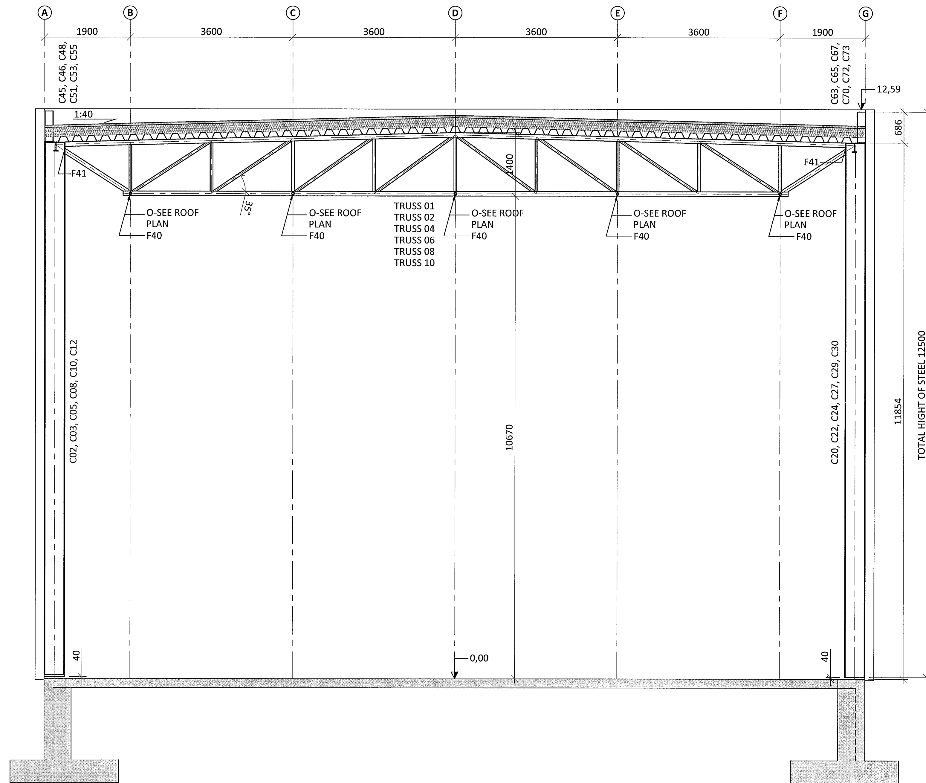
SECTION VIEW GRIDLINES 2,3,5,8,10,12 SC1:50
