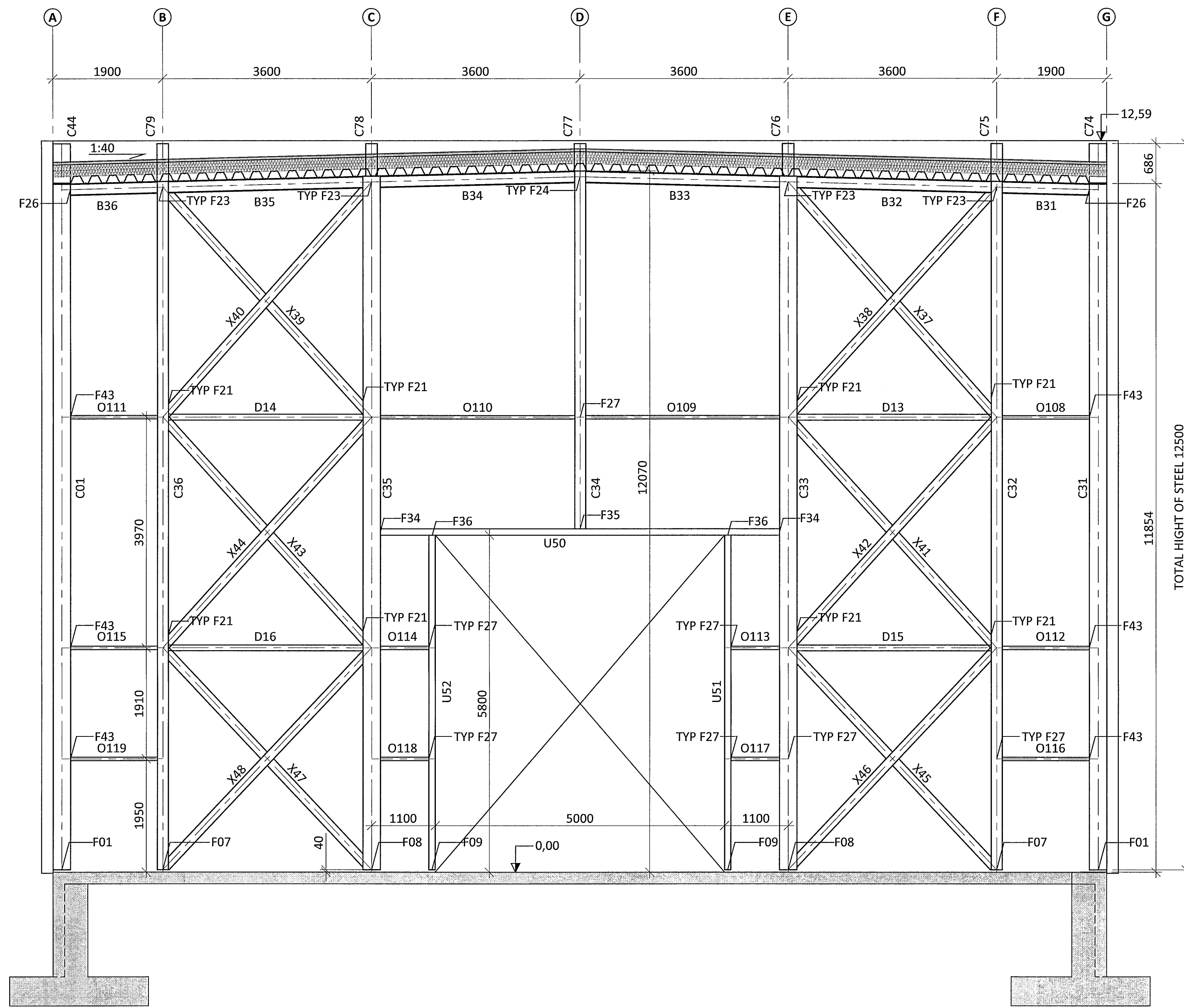
ELEVATION VIEW GRIDLINE 1 SC1:50
