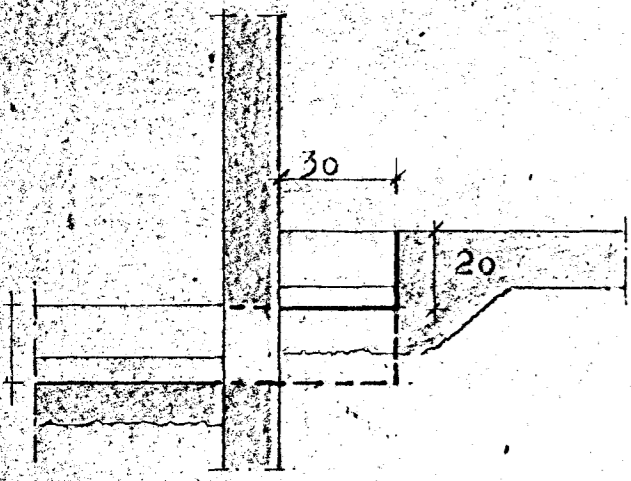
SNID - A 1:20
