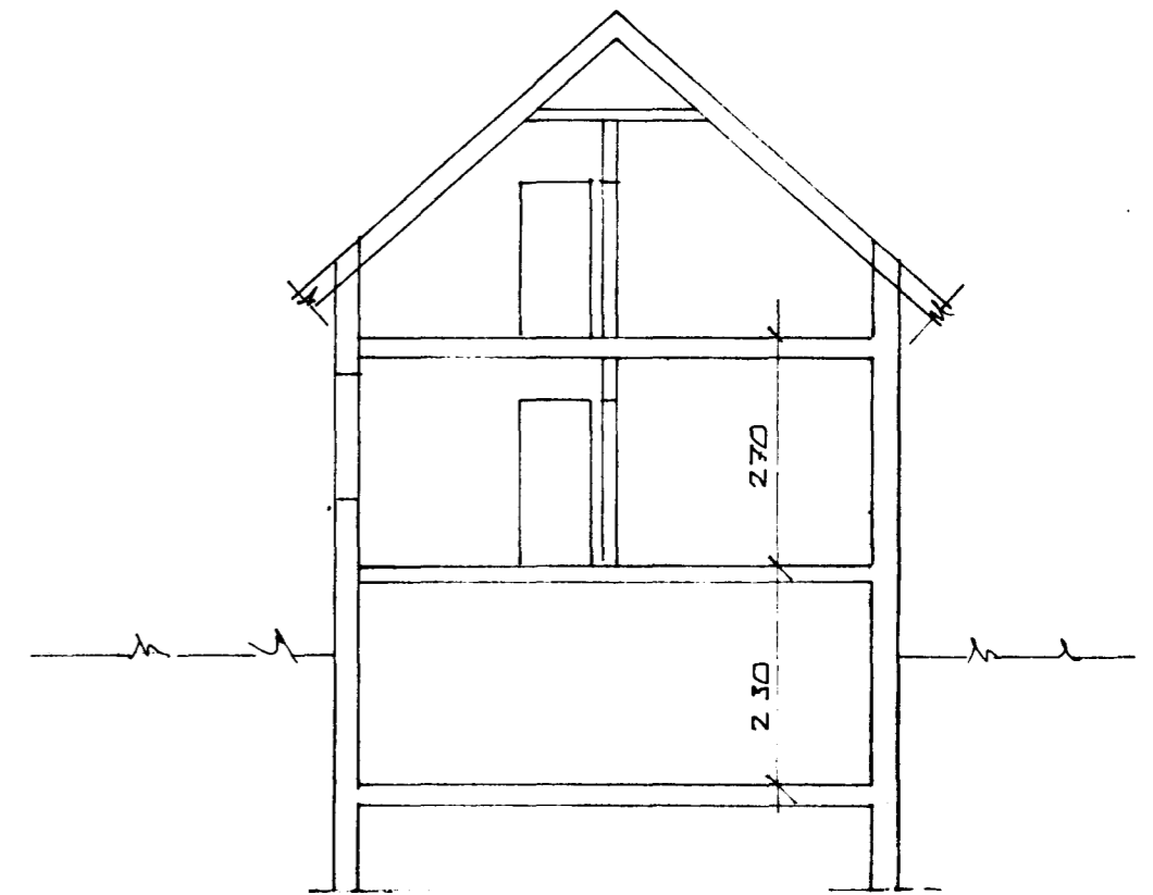
SNID A - A 1:100
