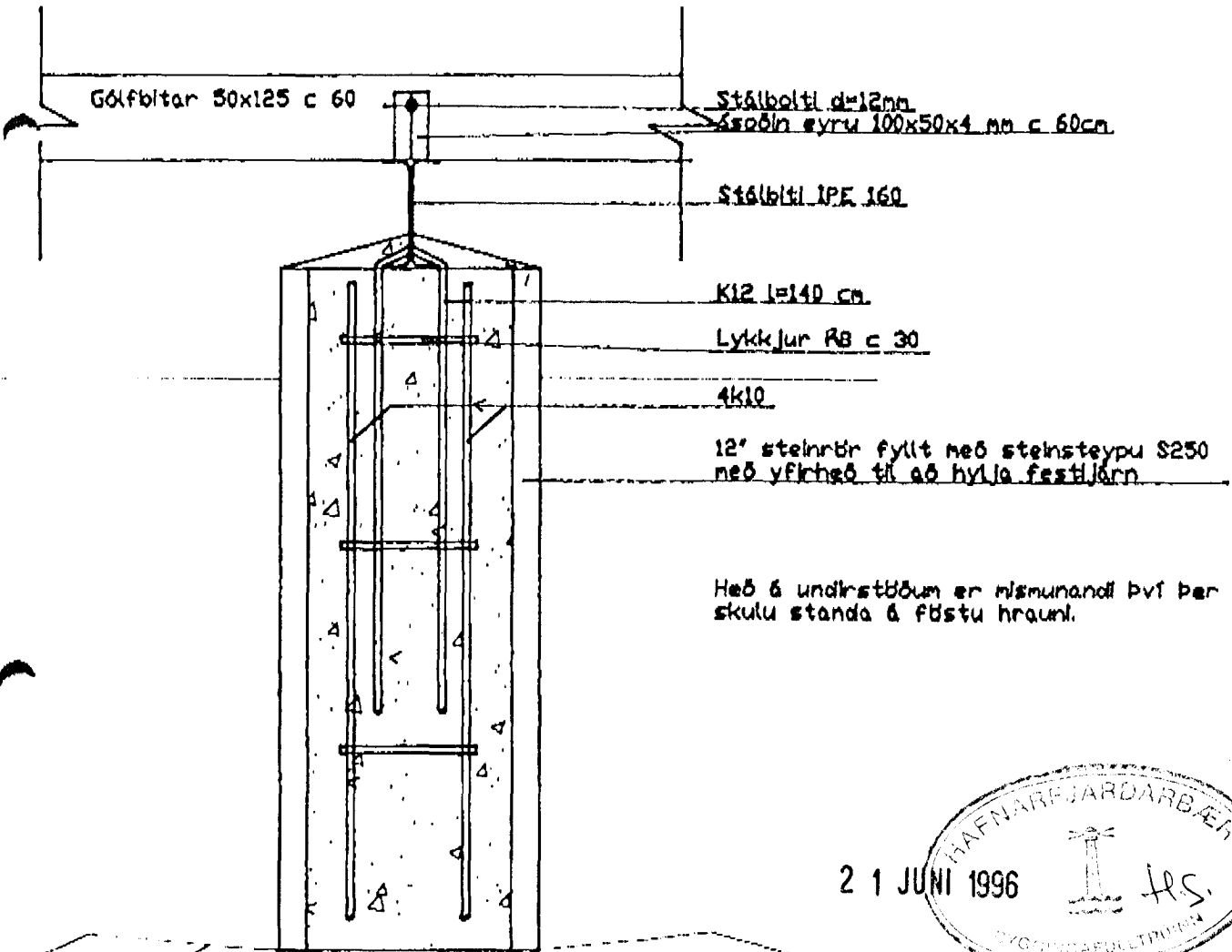
UNDIRSTAGA MKV 1:10
