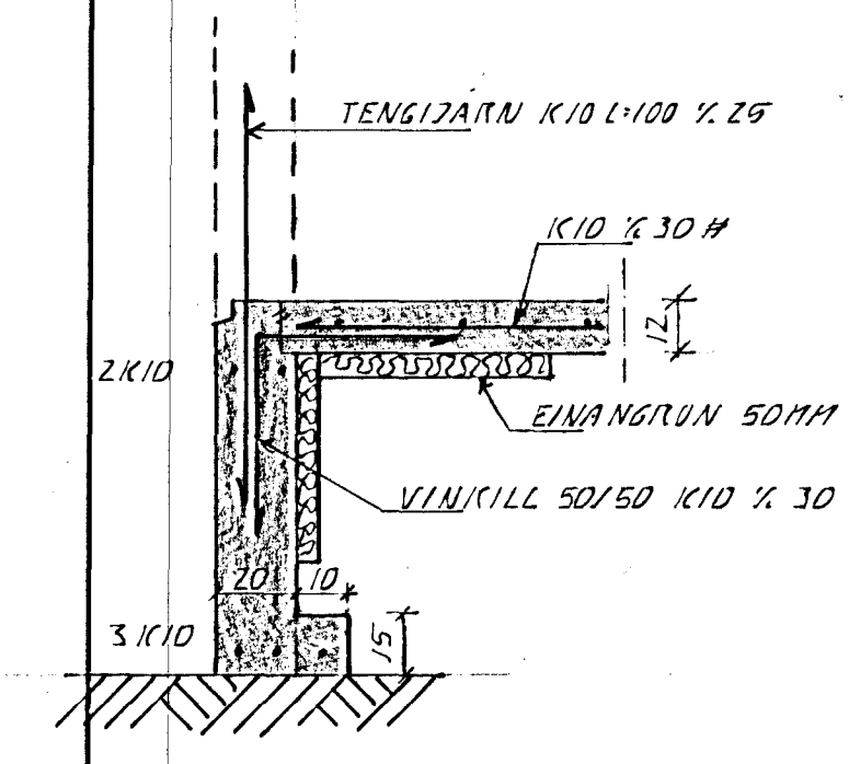
SNID 6, 1:20
