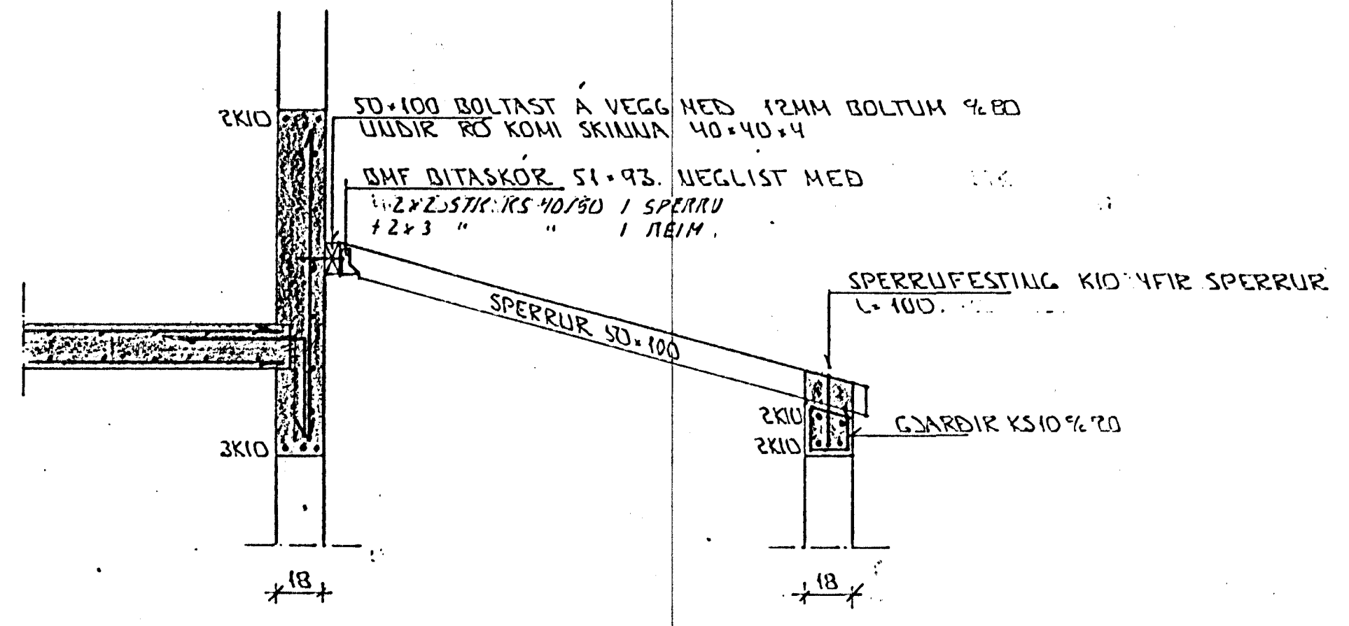
SNID 7-7 1:20
