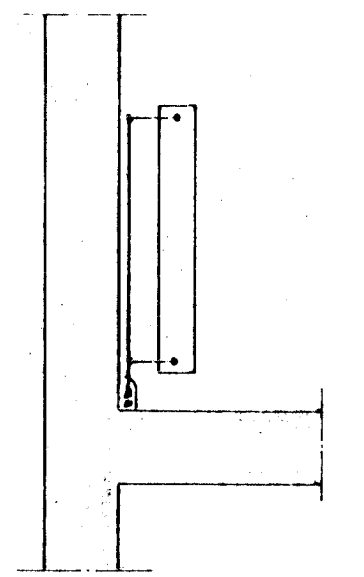
SNID B-B
