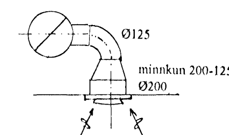
SNID C-C 1:20
