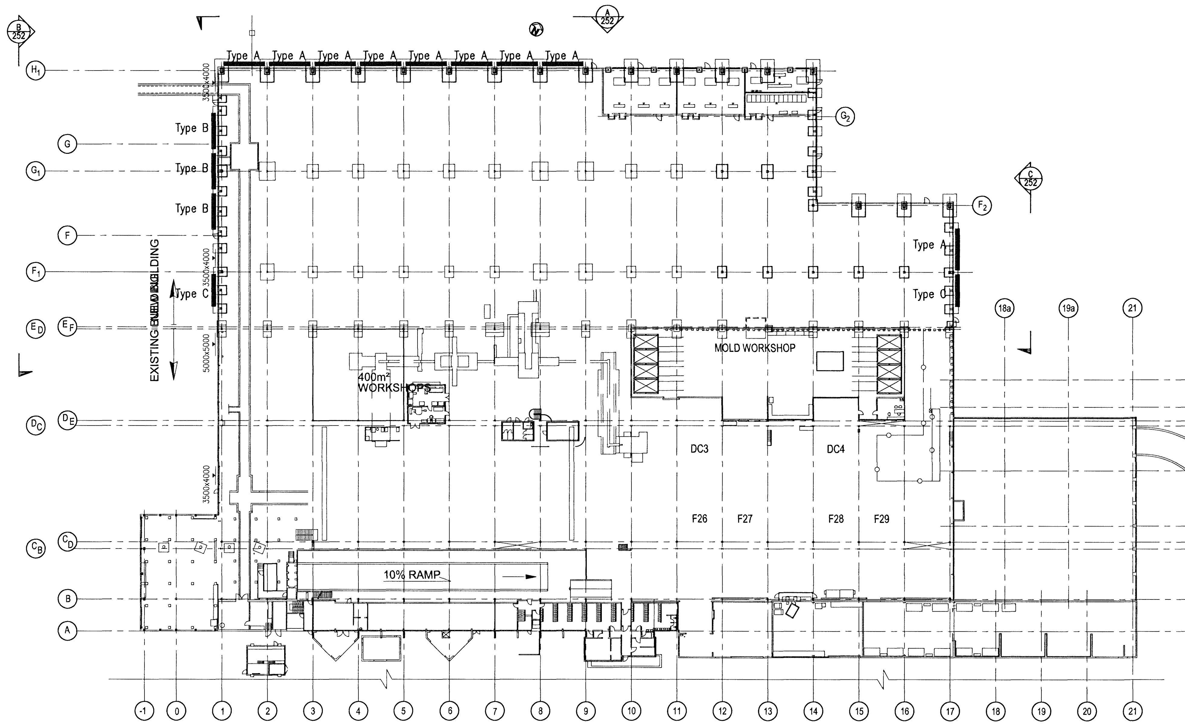
PLAN VIEW, 1:500
