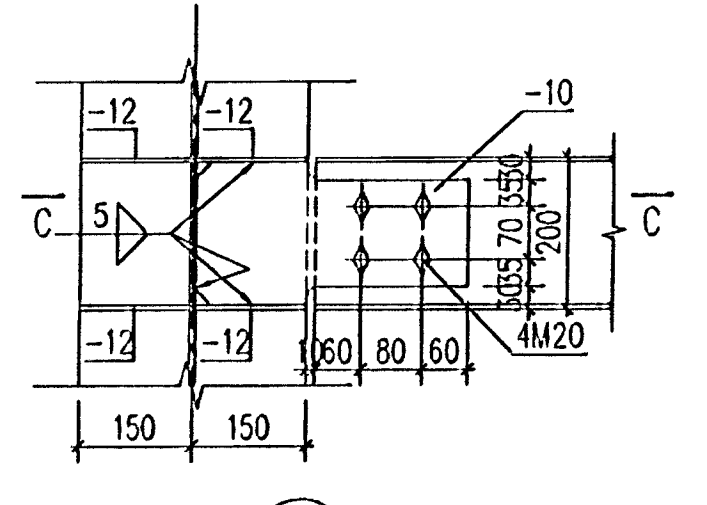
Scale 1:10
