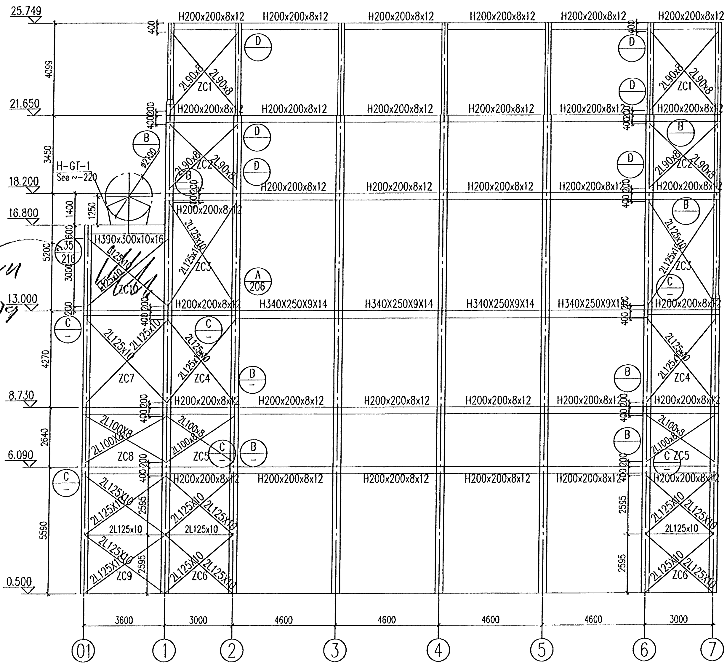
CONNECTIONS OF ANGLES ARE SHOWN ON DRAWINGS 214 AND 215
