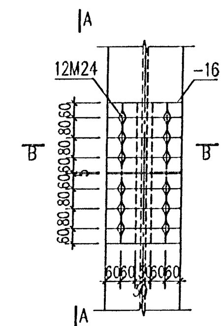
H390x300x10x16 拼接节点 Spliced joint of H390x300x10x16 Scale 1:15
