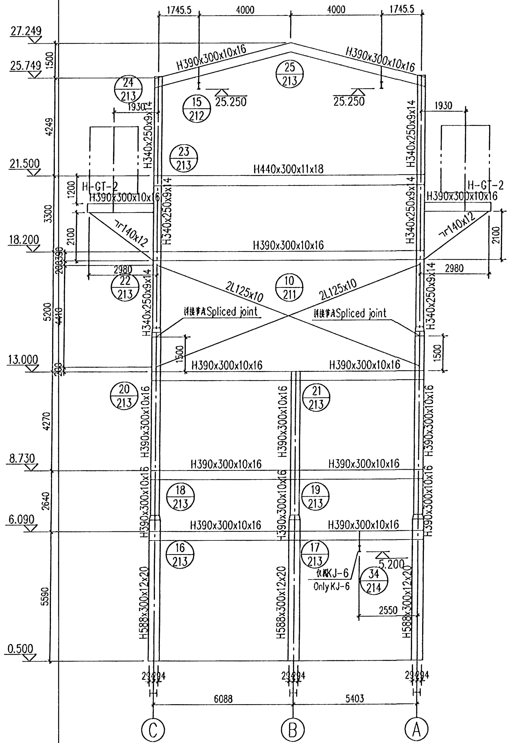
KJ-2 (KJ-6) Scale 1:100
