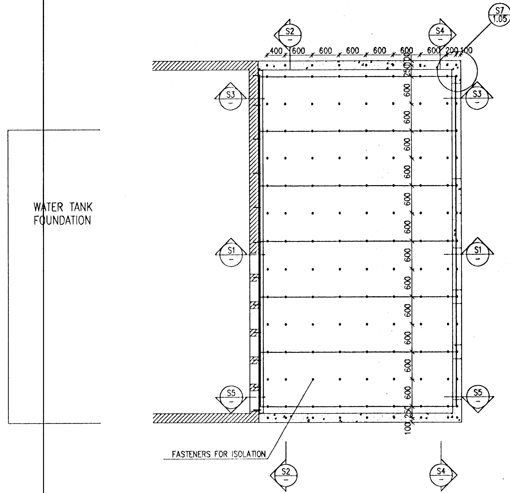
ROOF PLAN
