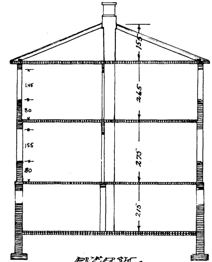
ÞVERSM.
