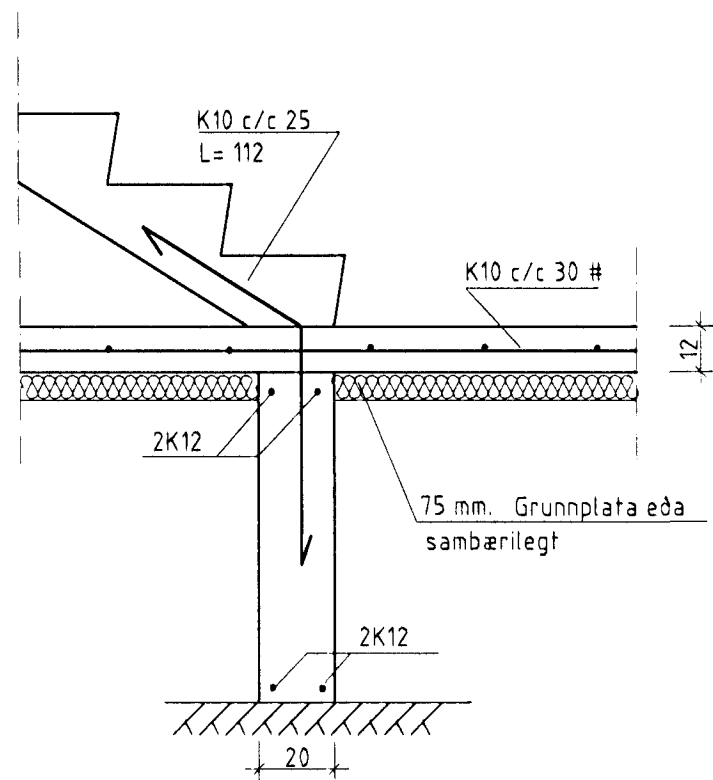
SNID E-E 1:20
