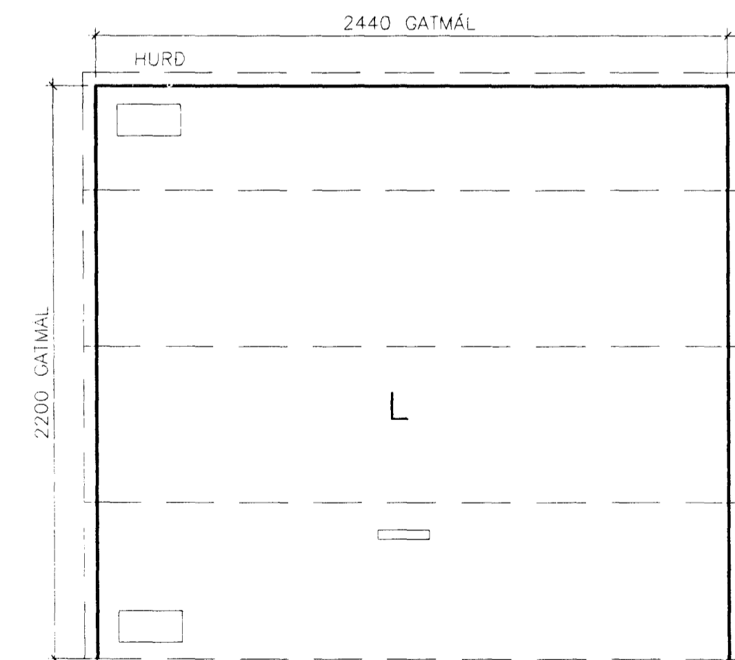
1 STK. BILGEYMSLUDYR, GATMDAL 2440X2200mm
