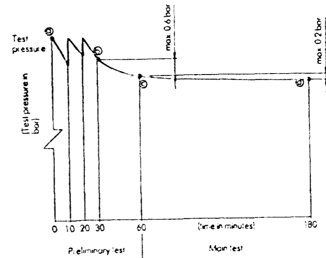
Pressure Test Diagram
