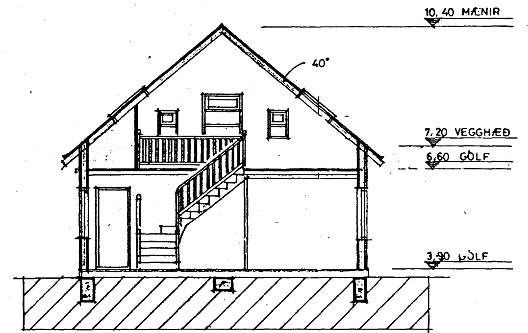
SNIB 1:100
