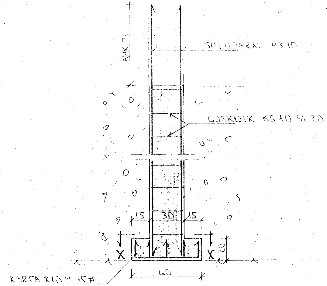
SNILA S1 x 1:20
