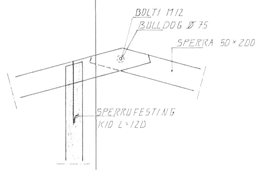
SNID 3.1:20
