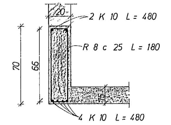
SNID B 1:20
