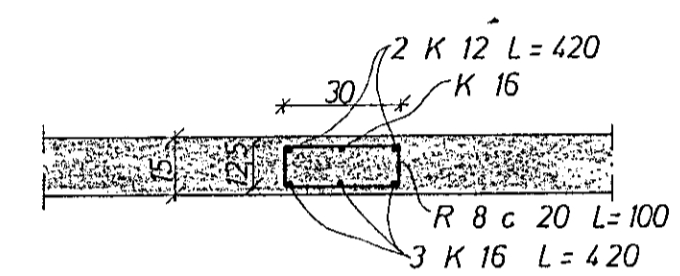
SNID C 1:20
