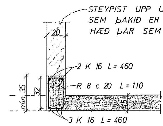
SNID A 1:20
