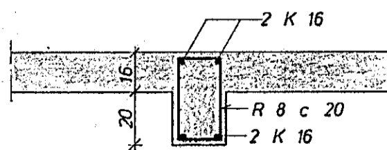
SNID A 1:20
