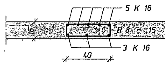
SNID B 1:20
