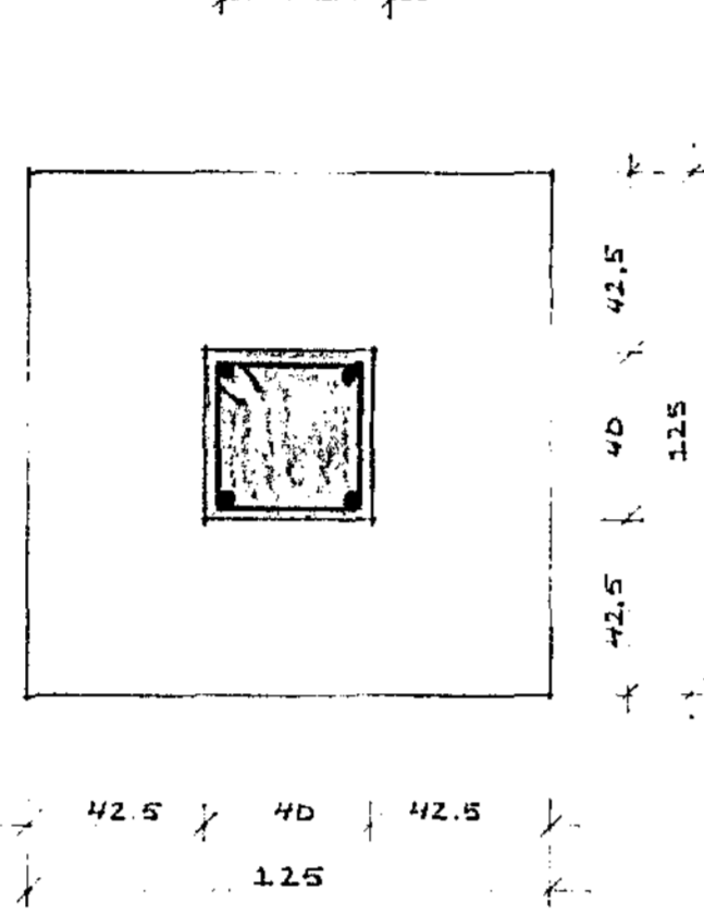
UNDIRSTADA U2 1:20
