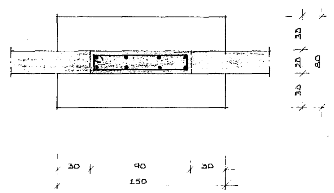
UNDIRSTADA U4 1:20
