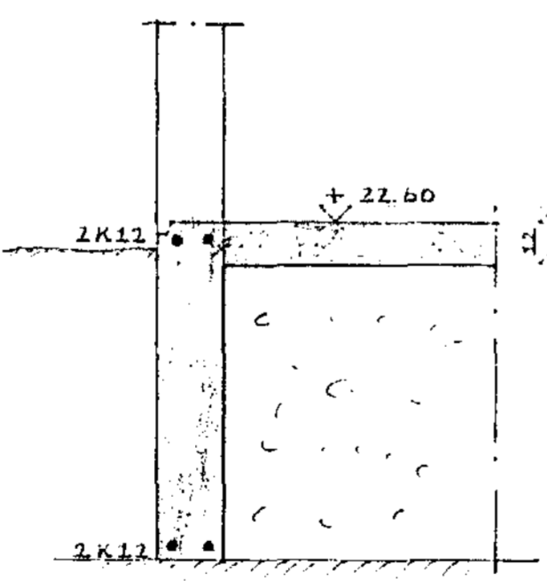
SNID C-C 1:20
