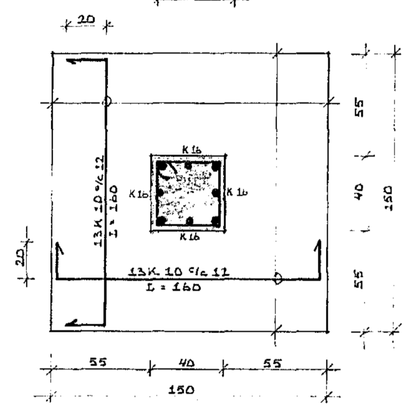
UNDIRSTADA U1 1:20
