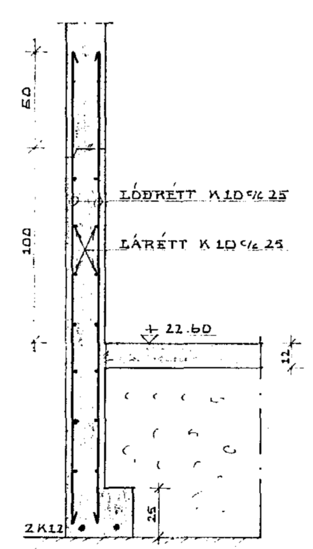
SNID E-E 1:20
