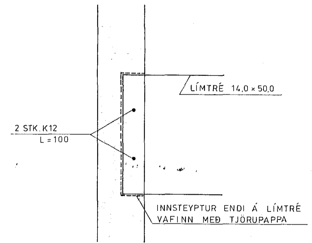
SNID 12-12 1:10
