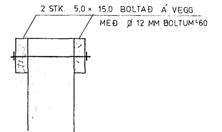
SNID 11-11 1:10
