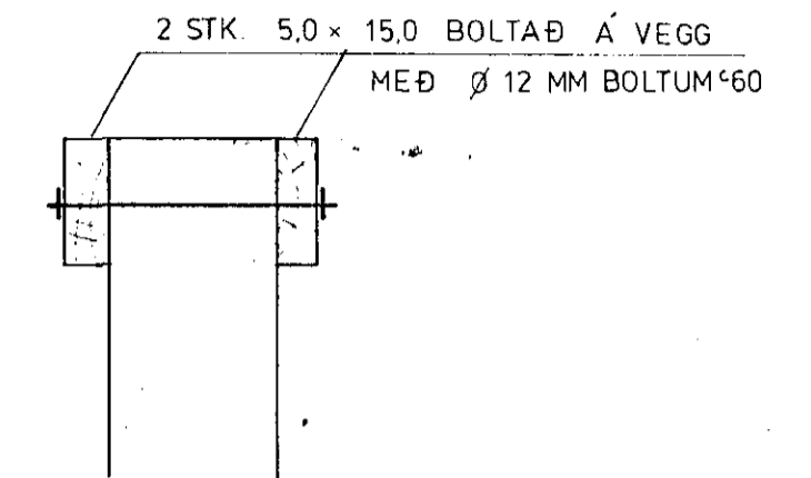
SNID 11-11 1:10
