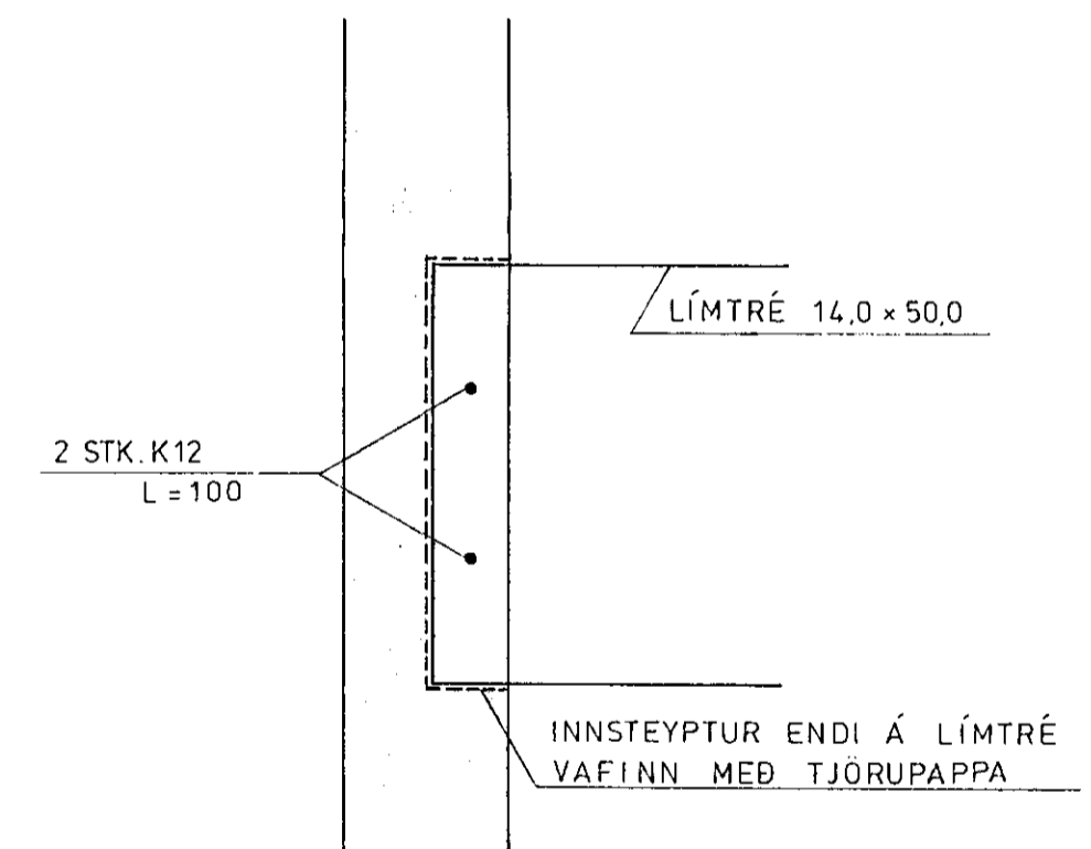
SNID 12-12 1:10
