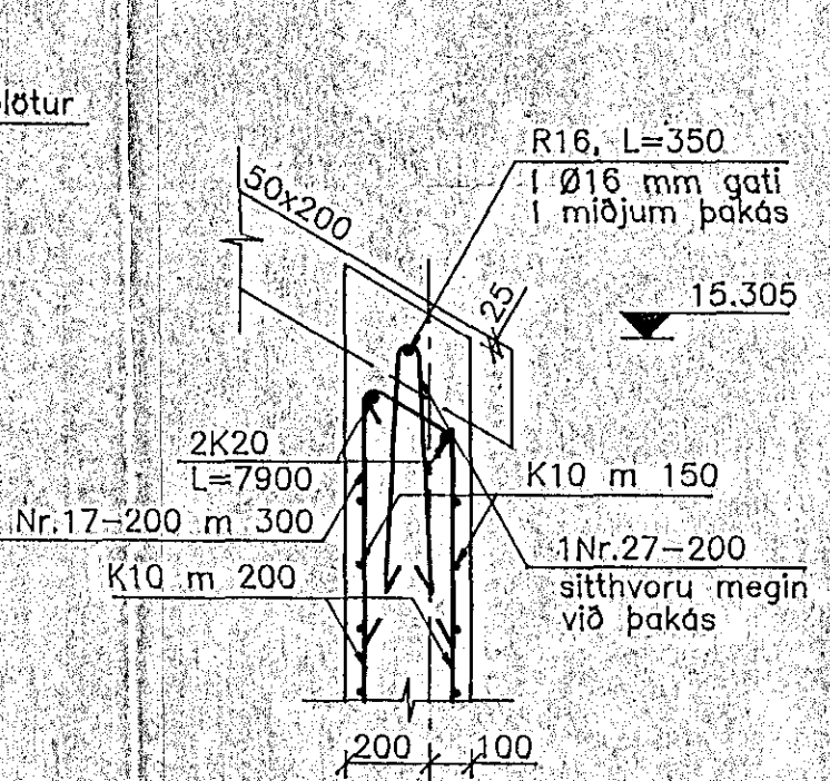
3 SNID 200/236 236 M 1:20
