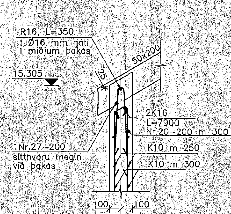
1 SNID 200/236 236 M 1:20
