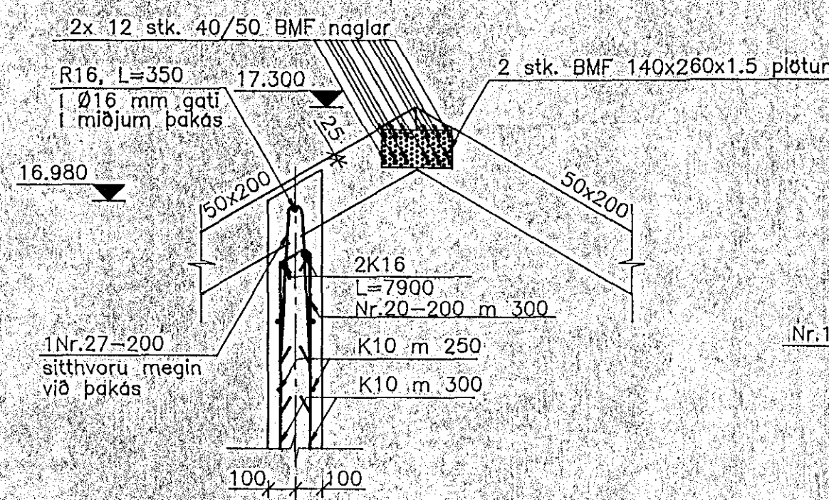
2 SNID 200/236 236 M 1:20
