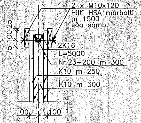
4 SNID 236/236 M 1:20
