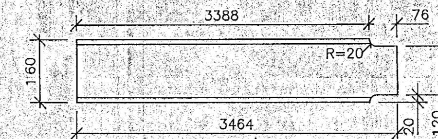
S26 HE160B, L=3464, 2 stk. M. 1:10
