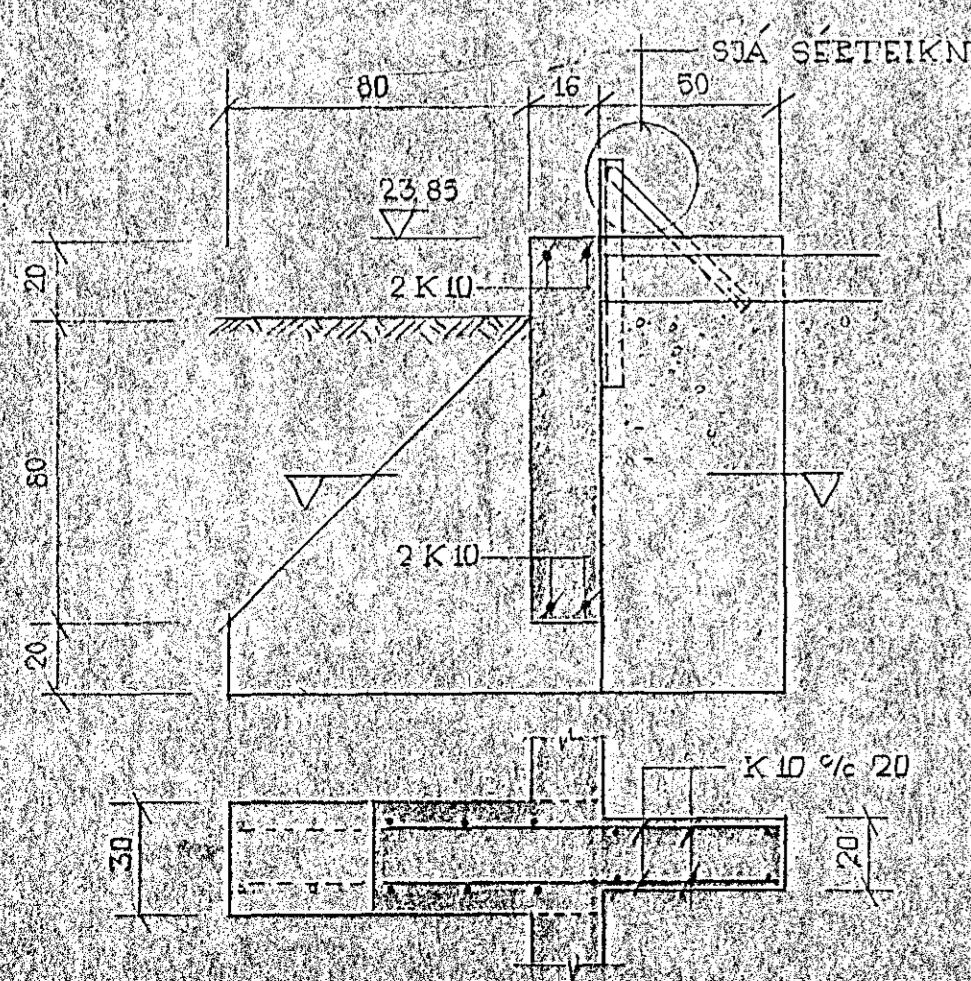
UNDIRSTADA U1 1:20
