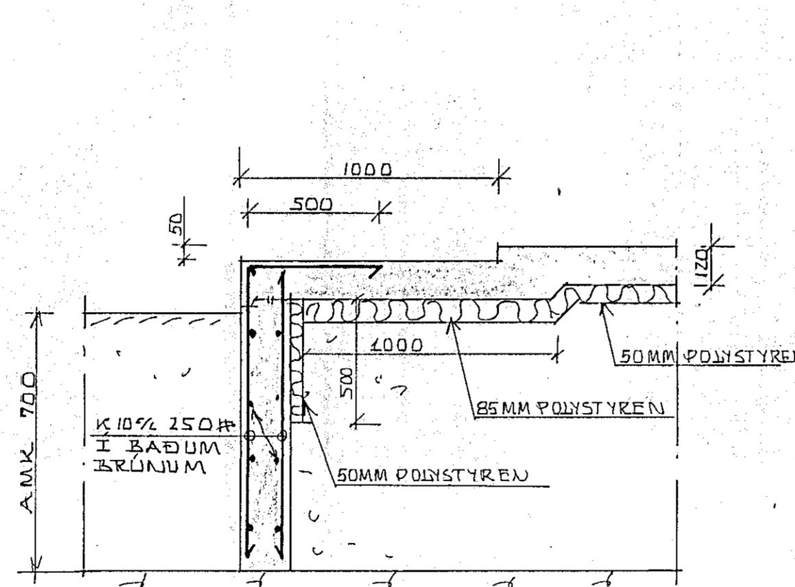
SNID C-C 1:20
