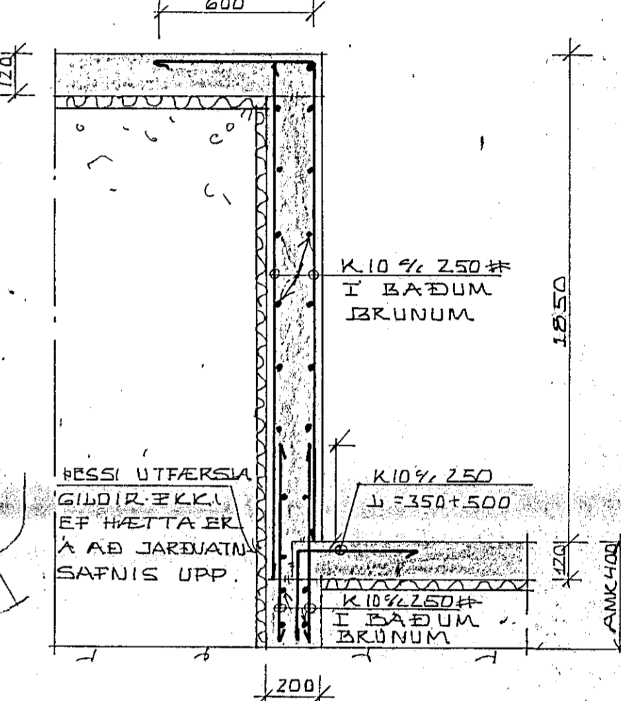
SNID H-H 1:20
