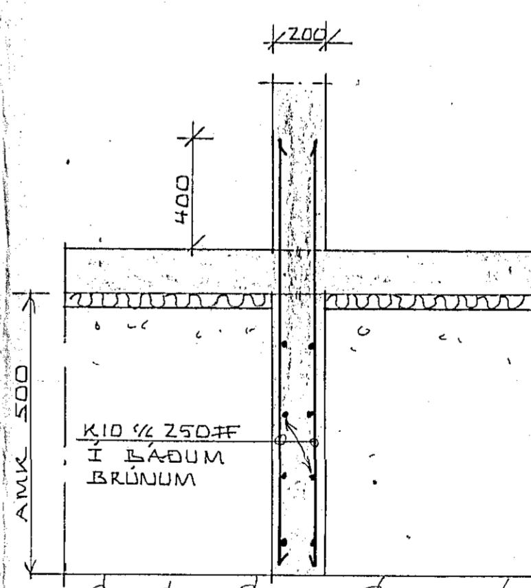
SNID F-F 1:20
