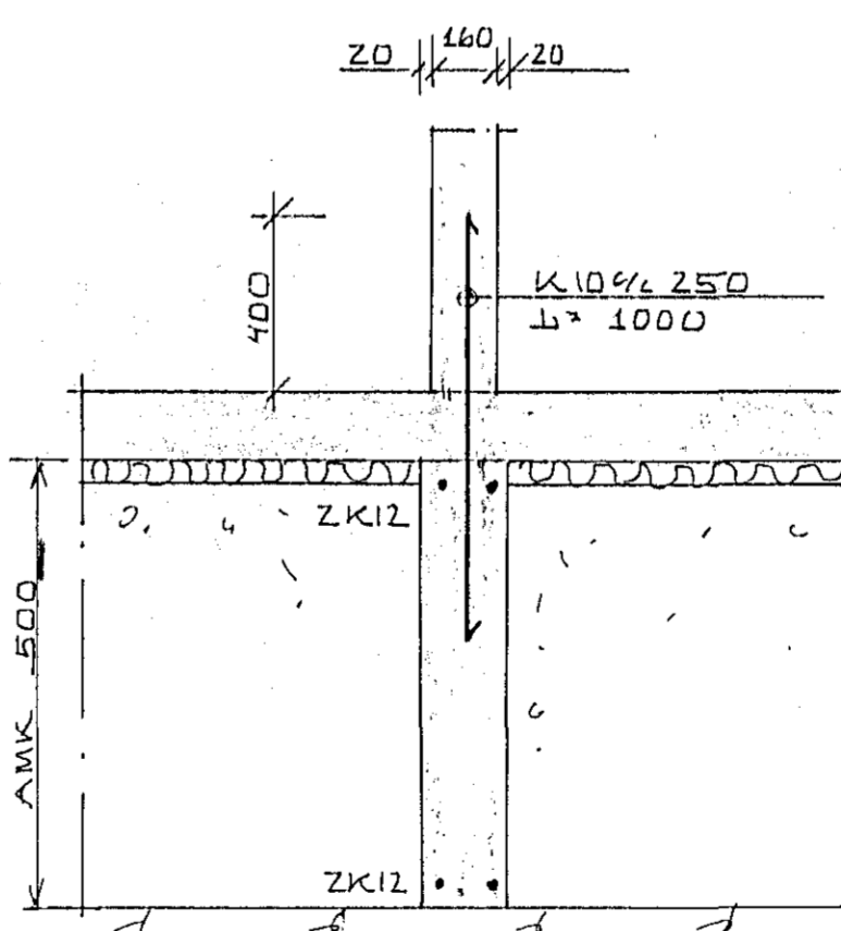
SNID E-E 1:20
