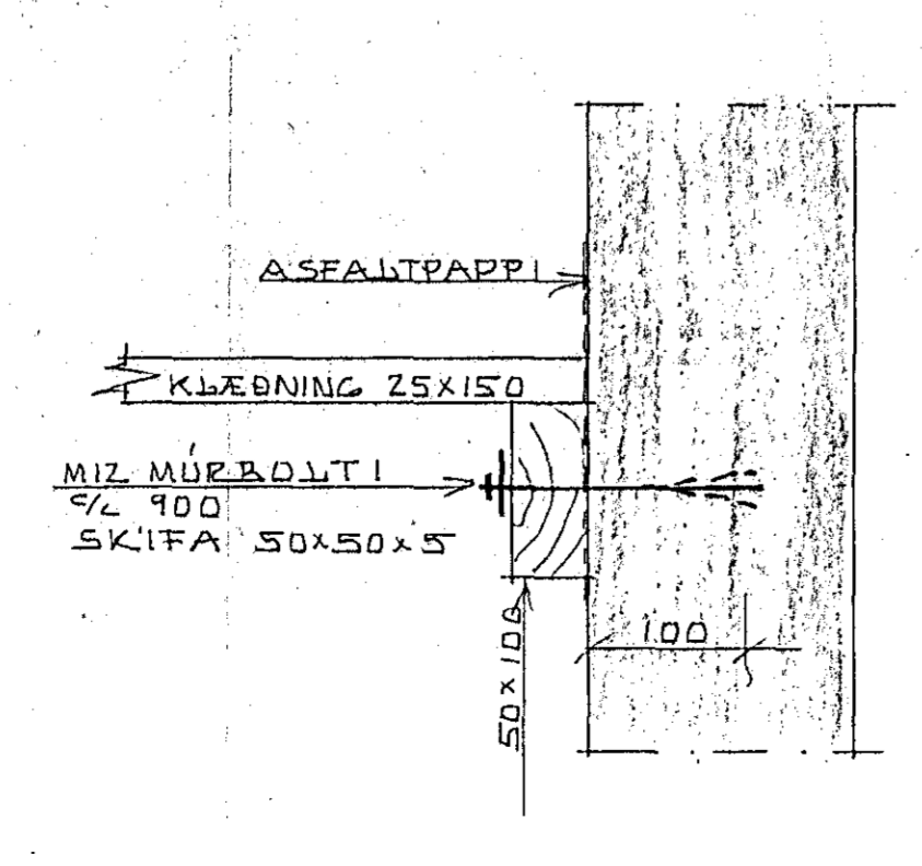
SNID C-C 1:5
